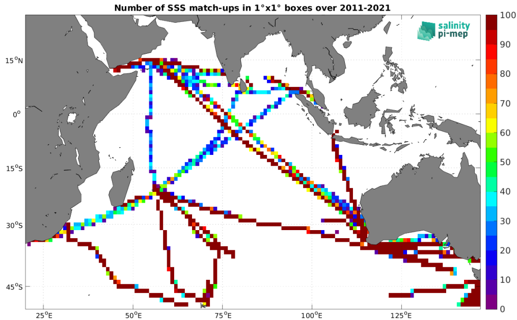
Figure 5: Number of SSS match-ups between TSG (LEGOS-DM) SSS and the SMOS SSS L3 v2 - 9-Days (BEC) SSS product for the Indian Ocean Pi-MEP region over 1^\circ \times 1^\circ boxes and for the full satellite product period.
