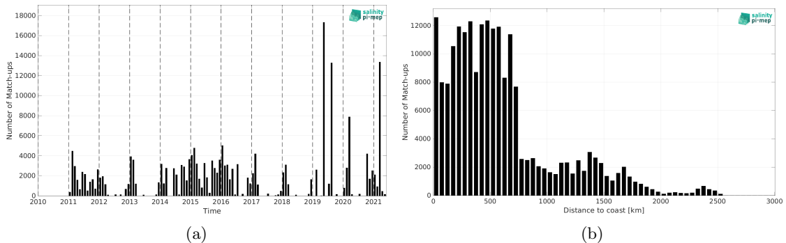
Figure 2: Number of match-ups between TSG (LEGOS-DM) and SMOS SSS L3 v2 - 9-Days (BEC) SSS as a function of time (a) and as function of the distance to coast (b) over the Indian Ocean Pi-MEP region and for the full satellite product period.
