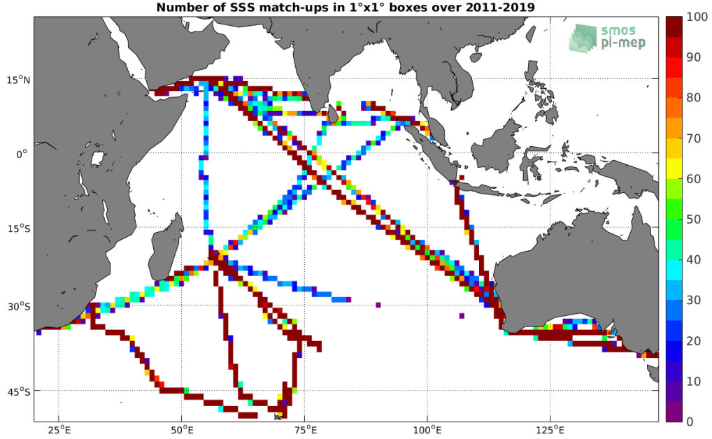
Figure 4: Number of SSS match-ups between TSG (LEGOS-DM) SSS and the SMOS SSS L3 v2 - 9-Days (BEC) SSS product for the Indian Ocean Pi-MEP region over 1^\circ \times 1^\circ boxes and for the full satellite product period.
