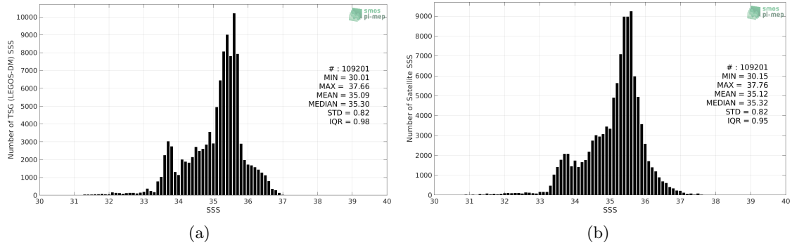
Figure 2: Histograms of SSS from TSG (LEGOS-DM) (a) and SMOS SSS L3 v2 - 9-Days (BEC) (b) considering all match-up pairs per bins of 0.1 over the Indian Ocean Pi-MEP region and for the full satellite product period.
