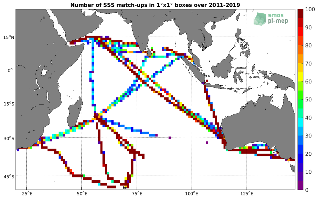
Figure 4: Number of SSS match-ups between TSG (LEGOS-DM) SSS and the SMOS SSS L3 v2 - 9-Days (BEC) SSS product for the Indian Ocean Pi-MEP region over 1^\circ \times 1^\circ boxes and for the full satellite product period.
