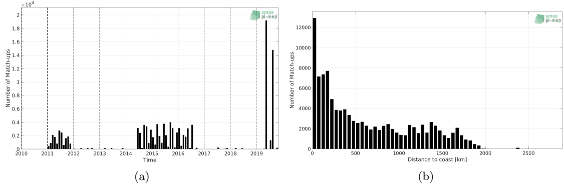
Figure 1: Number of match-ups between TSG (LEGOS-DM) and SMOS SSS L3 v2 - 9-Days (BEC) SSS as a function of time (a) and as function of the distance to coast (b) over the Indian Ocean Pi-MEP region and for the full satellite product period.
