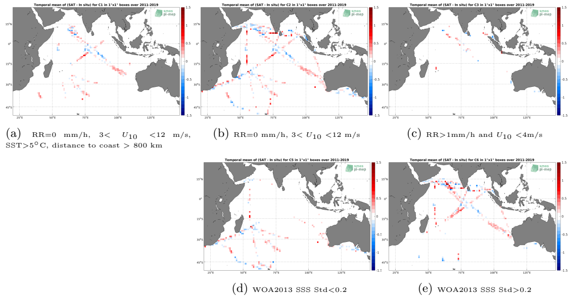
Figure 12: Temporal mean gridded over spatial boxes of size 1^\circ \times 1^\circ of \Delta SSS (SMOS SSS L3 v2 - 9-Days (BEC) - TSG (LEGOS-DM)) for 5 different subdatasets corresponding to: RR=0 mm/h, 3 < U_{10} < 12 m/s, SST > 5^\circ C , distance to coast > 800 km (a), RR=0 mm/h, 3 < U_{10} < 12 m/s (b), RR > 1 mm/h and U_{10} < 4 m/s (c), WOA2013 SSS Std < 0.2 (d), WOA2013 SSS Std > 0.2 (e).
