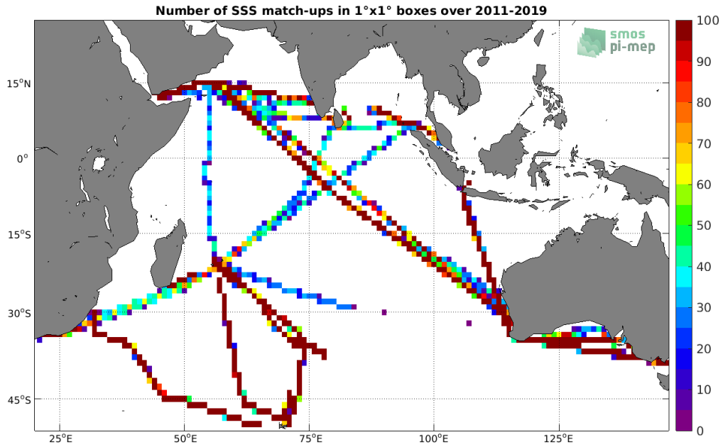
Figure 4: Number of SSS match-ups between TSG (LEGOS-DM) SSS and the SMOS SSS L3 v2 - 9-Days (BEC) SSS product for the Indian Ocean Pi-MEP region over 1°x1° boxes and for the full satellite product period.
