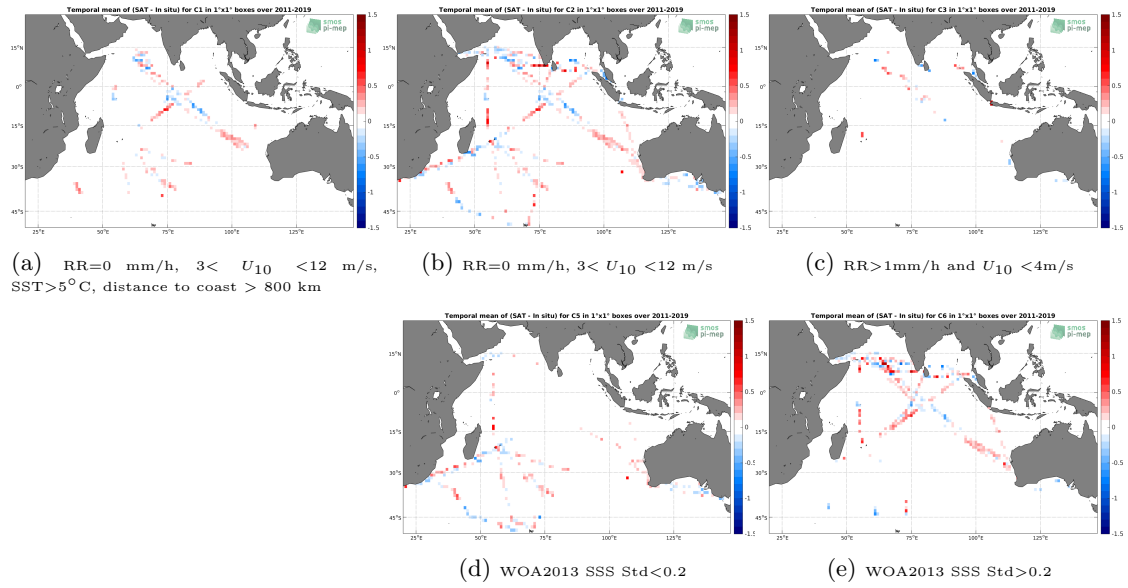
Figure 12: Temporal mean gridded over spatial boxes of size 1^\circ \times 1^\circ of \Delta SSS (SMOS L3 v2 - 9-Days (BEC) - TSG (LEGOS-DM)) for 5 different subdatasets corresponding to: RR=0 mm/h, 3 < U_{10} < 12 m/s, SST > 5^\circ\text{C} , distance to coast > 800 km (a), RR=0 mm/h, 3 < U_{10} < 12 m/s (b), RR > 1 mm/h and U_{10} < 4 m/s (c), WOA2013 SSS Std < 0.2 (d), WOA2013 SSS Std > 0.2 (e).
