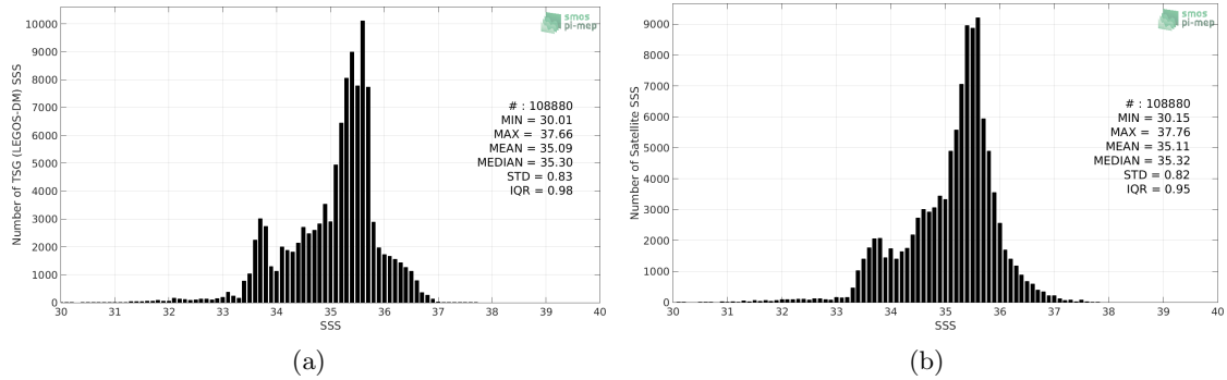
Figure 2: Histograms of SSS from TSG (LEGOS-DM) (a) and SMOS L3 v2 - 9-Days (BEC) (b) considering all match-up pairs per bins of 0.1 over the Indian Ocean Pi-MEP region and for the full satellite product period.
