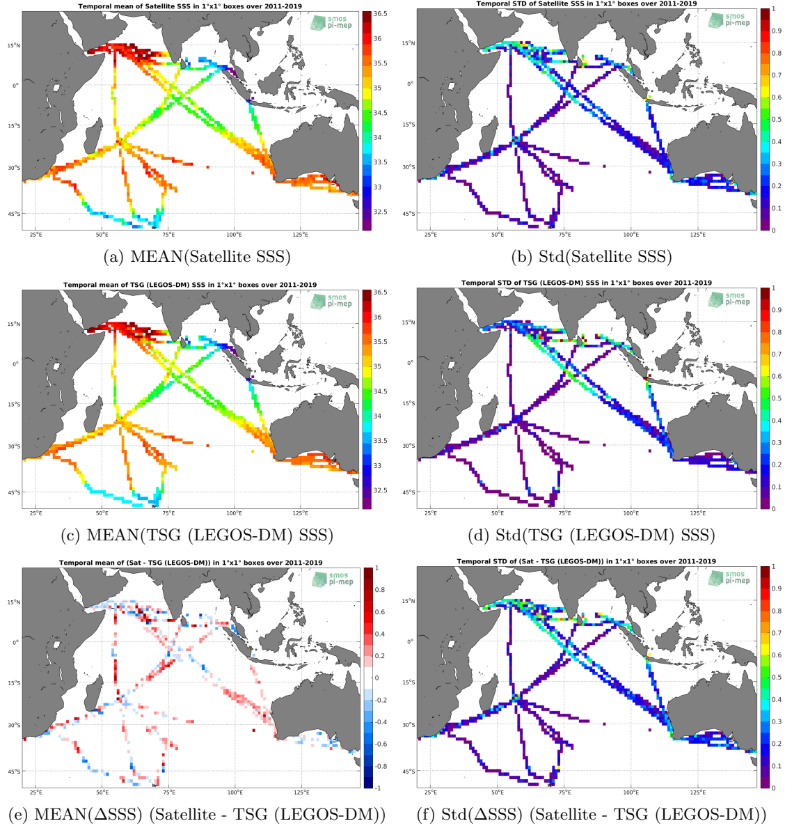
Figure 6: Temporal mean (left) and Std (right) of SSS from SMOS L3 v2 - 9-Days (BEC) (top), TSG (LEGOS-DM) (middle), and of \Delta SSS (Satellite - TSG (LEGOS-DM)). Only match-up pairs are used to generate these maps.
