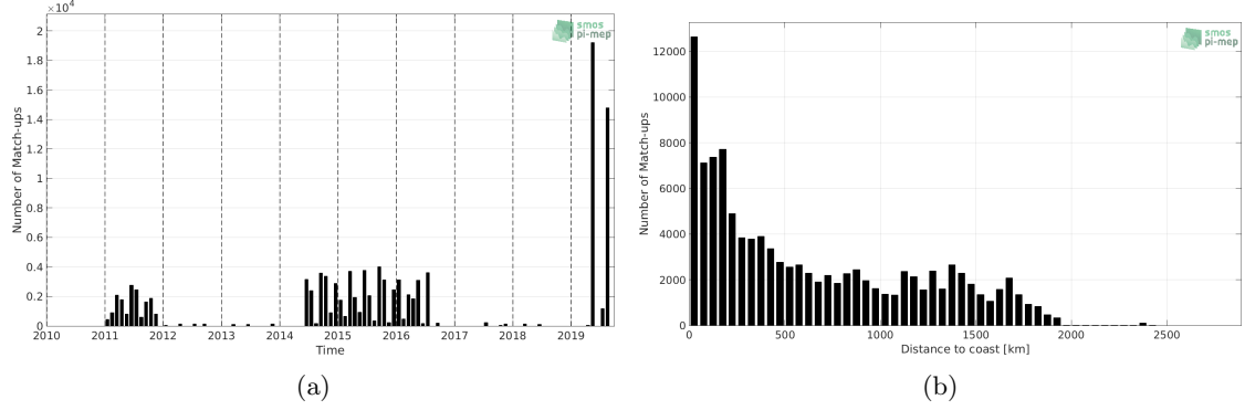
Figure 1: Number of match-ups between TSG (LEGOS-DM) and SMOS L3 v2 - 9-Days (BEC) SSS as a function of time (a) and as function of the distance to coast (b) over the Indian Ocean Pi-MEP region and for the full satellite product period.
