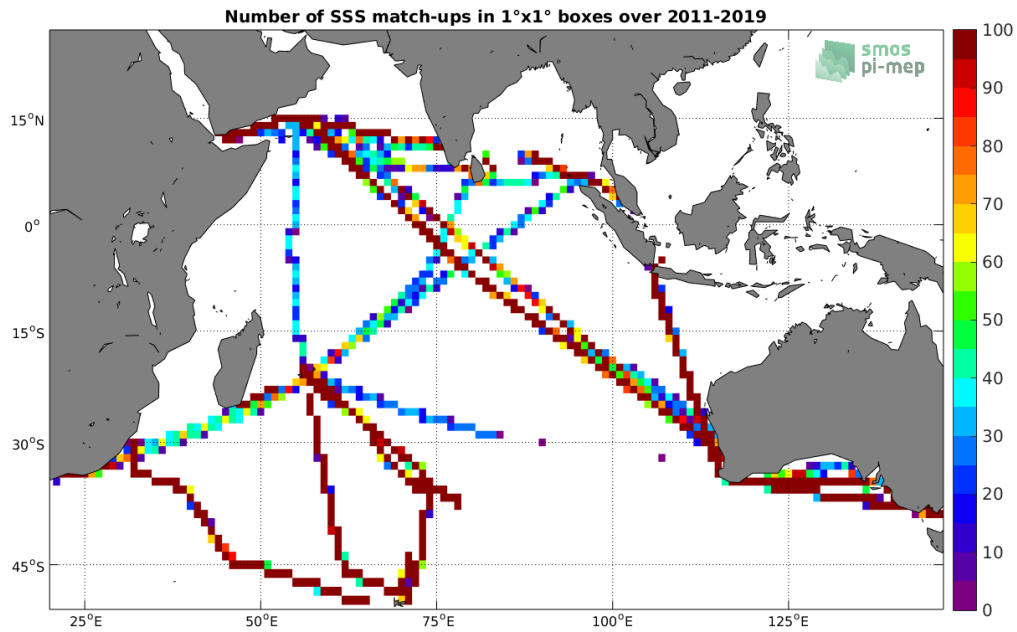
Figure 4: Number of SSS match-ups between TSG (LEGOS-DM) SSS and the SMOS L3 v2 - 9-Days (BEC) SSS product for the Indian Ocean Pi-MEP region over 1°x1° boxes and for the full satellite product period.
