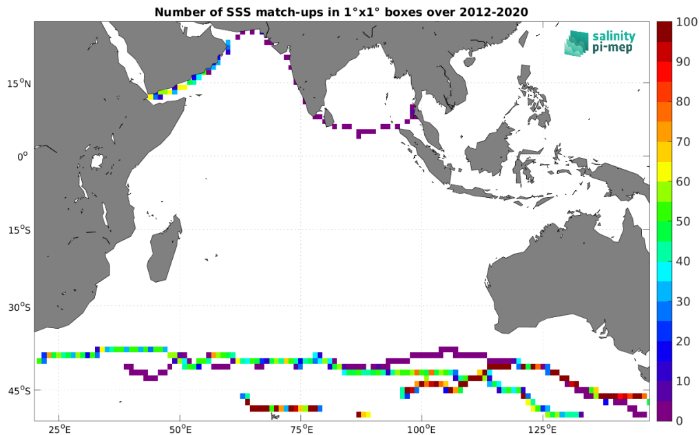
Figure 5: Number of SSS match-ups between TSG (GOSUD-Sailing-ship) SSS and the SMOS SSS L3 v2 - 9-Days (BEC) SSS product for the Indian Ocean Pi-MEP region over 1^\circ \times 1^\circ boxes and for the full satellite product period.
