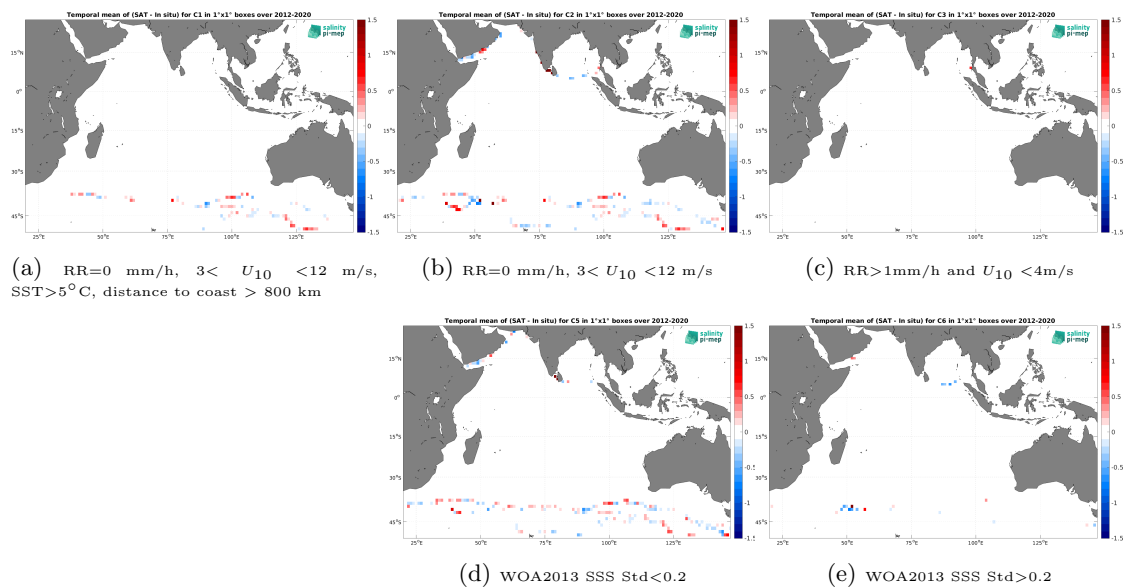
Figure 14: Temporal mean gridded over spatial boxes of size 1^\circ \times 1^\circ of \Delta\text{SSS} (SMOS SSS L3 v2 - 9-Days (BEC) - TSG (GOSUD-Sailing-ship)) for 5 different subdatasets corresponding to:RR=0 mm/h, 3 < U_{10} < 12 m/s, SST >5^\circ\text{C} , distance to coast > 800 km (a), RR=0 mm/h, 3 < U_{10} < 12 m/s (b), RR >1 mm/h and U_{10} < 4 m/s (c), WOA2013 SSS Std <0.2 (d), WOA2013 SSS Std >0.2 (e).
