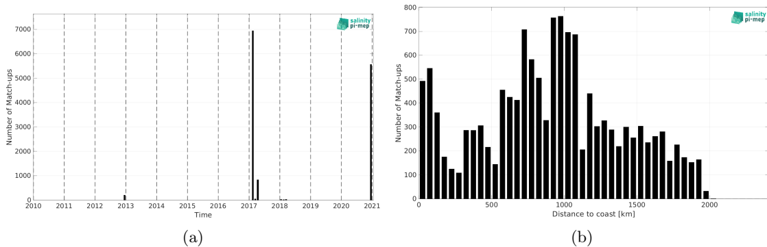
Figure 2: Number of match-ups between TSG (GOSUD-Sailing-ship) and SMOS SSS L3 v2 - 9-Days (BEC) SSS as a function of time (a) and as function of the distance to coast (b) over the Indian Ocean Pi-MEP region and for the full satellite product period.
