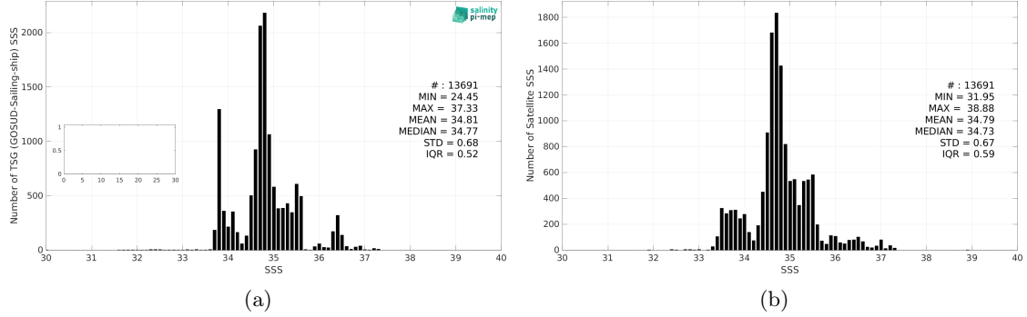
Figure 3: Histograms of SSS from TSG (GOSUD-Sailing-ship) (a) and SMOS SSS L3 v2 - 9-Days (BEC) (b) considering all match-up pairs per bins of 0.1 over the Indian Ocean Pi-MEP region and for the full satellite product period.
