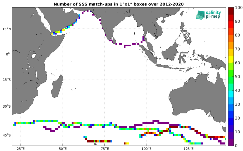
Figure 5: Number of SSS match-ups between TSG (GOSUD-Sailing-ship) SSS and the SMOS SSS L3 v2 - 9-Days (BEC) SSS product for the Indian Ocean Pi-MEP region over 1^\circ \times 1^\circ boxes and for the full satellite product period.
