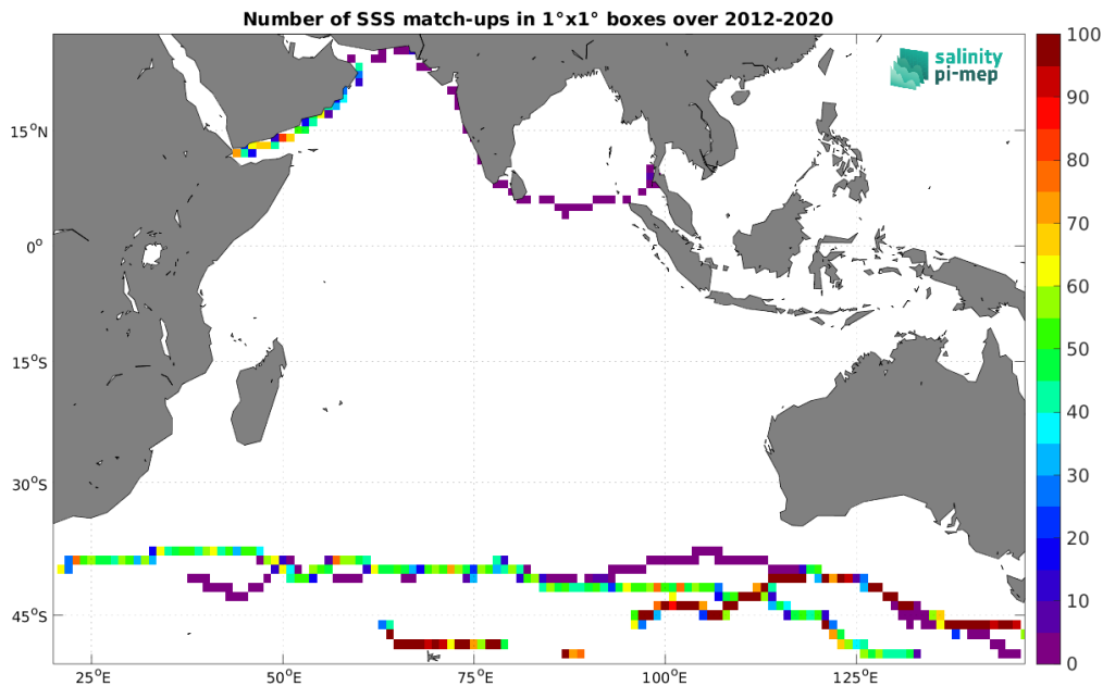
Figure 4: Number of SSS match-ups between TSG (GOSUD-Sailing-ship) SSS and the SMOS SSS L3 v2 - 9-Days (BEC) SSS product for the Indian Ocean Pi-MEP region over 1^\circ \times 1^\circ boxes and for the full satellite product period.
