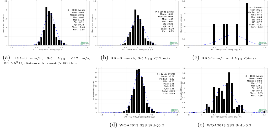
Figure 13: Normalized histogram of \Delta SSS (SMOS SSS L3 v2 - 9-Days (BEC) - TSG (GOSUD-Sailing-ship)) for 5 different subdatasets corresponding to: RR=0 mm/h, 3 < U_{10} < 12 m/s, SST > 5°C, distance to coast > 800 km (a), RR=0 mm/h, 3 < U_{10} < 12 m/s (b), RR > 1mm/h and U_{10} < 4 m/s (c), WOA2013 SSS Std < 0.2 (d), WOA2013 SSS Std > 0.2 (e).
