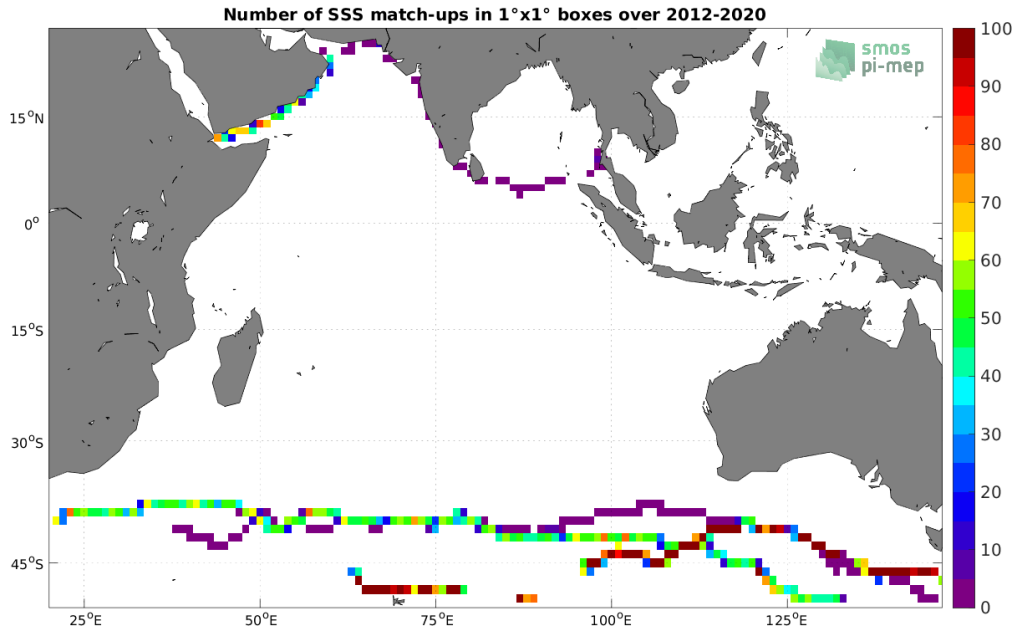
Figure 4: Number of SSS match-ups between TSG (GOSUD-Sailing-ship) SSS and the SMOS SSS L3 v2 - 9-Days (BEC) SSS product for the Indian Ocean Pi-MEP region over 1°x1° boxes and for the full satellite product period.
