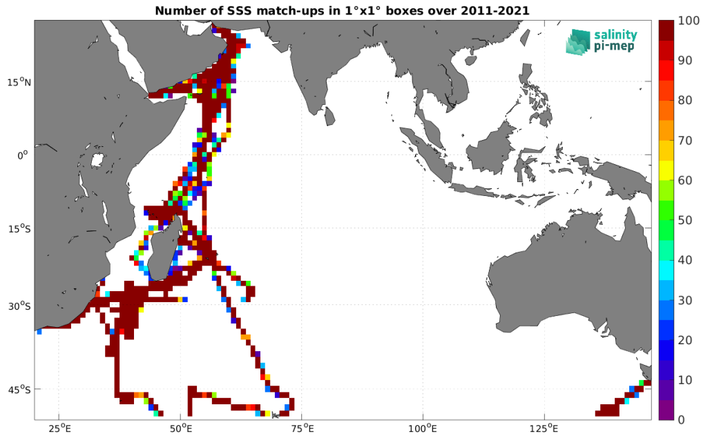
Figure 5: Number of SSS match-ups between TSG (GOSUD-Research-vessel) SSS and the SMOS SSS L3 v2 - 9-Days (BEC) SSS product for the Indian Ocean Pi-MEP region over 1^\circ \times 1^\circ boxes and for the full satellite product period.
