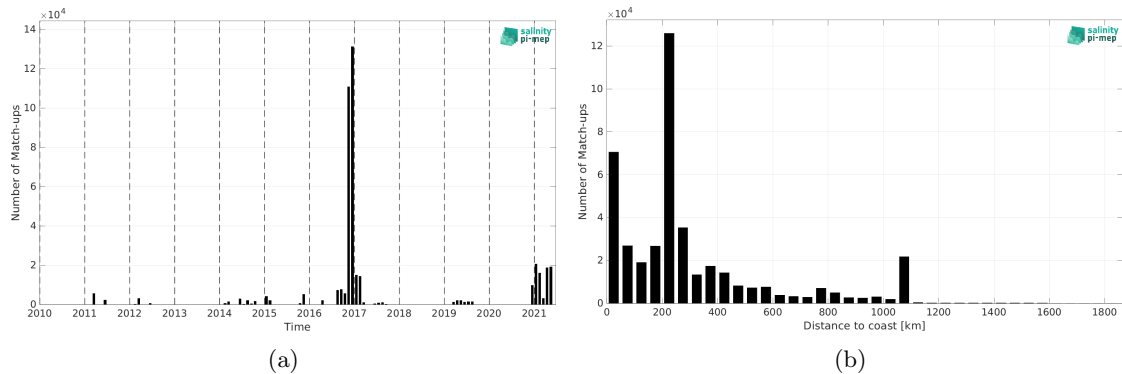
Figure 2: Number of match-ups between TSG (GOSUD-Research-vessel) and SMOS SSS L3 v2 - 9-Days (BEC) SSS as a function of time (a) and as function of the distance to coast (b) over the Indian Ocean Pi-MEP region and for the full satellite product period.
