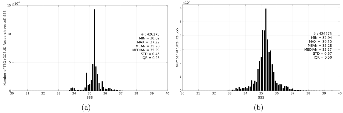
Figure 3: Histograms of SSS from TSG (GOSUD-Research-vessel) (a) and SMOS SSS L3 v2 - 9-Days (BEC) (b) considering all match-up pairs per bins of 0.1 over the Indian Ocean Pi-MEP region and for the full satellite product period.
