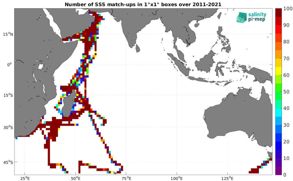
Figure 5: Number of SSS match-ups between TSG (GOSUD-Research-vessel) SSS and the SMOS SSS L3 v2 - 9-Days (BEC) SSS product for the Indian Ocean Pi-MEP region over 1^\circ \times 1^\circ boxes and for the full satellite product period.
