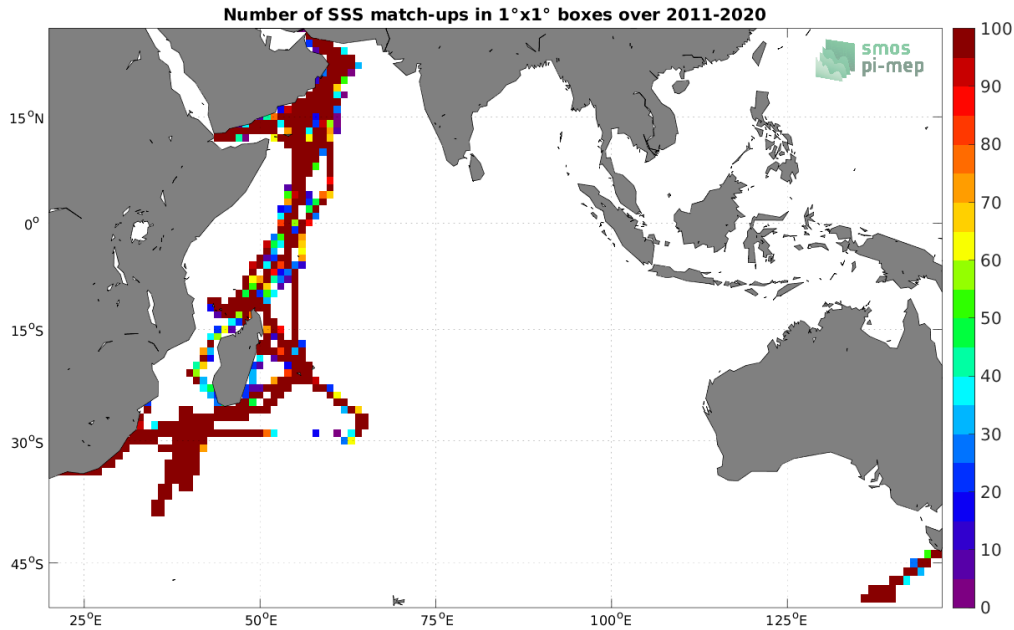
Figure 4: Number of SSS match-ups between TSG (GOSUD-Research-vessel) SSS and the SMOS SSS L3 v2 - 9-Days (BEC) SSS product for the Indian Ocean Pi-MEP region over 1^{\circ} \times 1^{\circ} boxes and for the full satellite product period.
