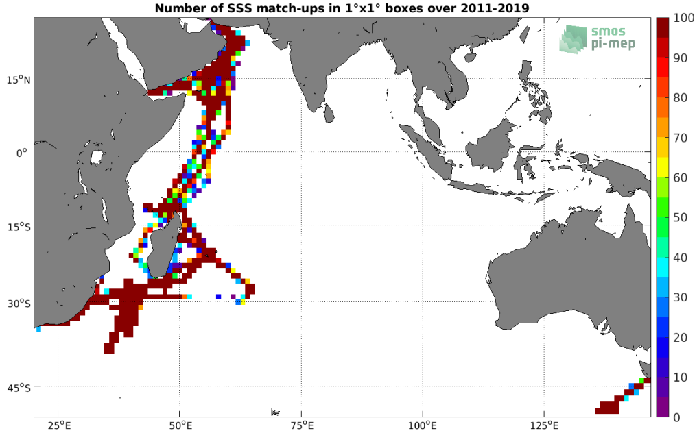
Figure 4: Number of SSS match-ups between TSG (GOSUD-Research-vessel) SSS and the SMOS SSS L3 v2 - 9-Days (BEC) SSS product for the Indian Ocean Pi-MEP region over 1^\circ \times 1^\circ boxes and for the full satellite product period.
