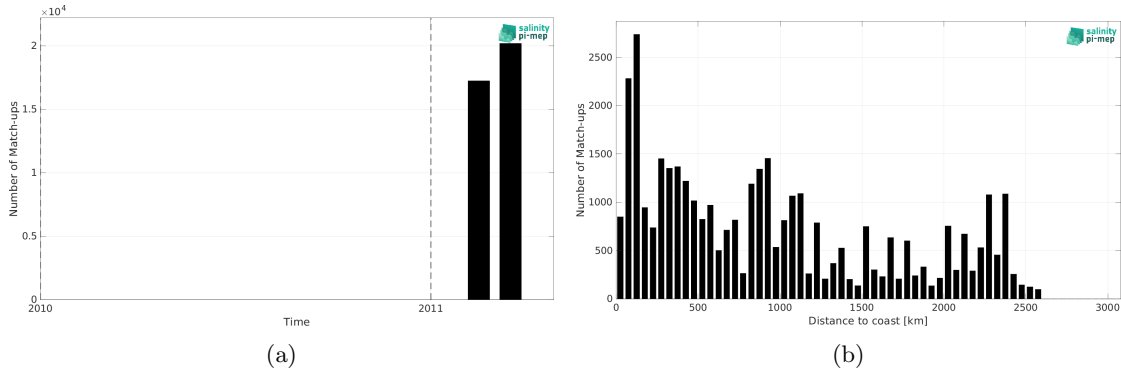
Figure 2: Number of match-ups between TSG (CSIC-UTM) and SMOS SSS L3 v2 - 9-Days (BEC) SSS as a function of time (a) and as function of the distance to coast (b) over the Indian Ocean Pi-MEP region and for the full satellite product period.
