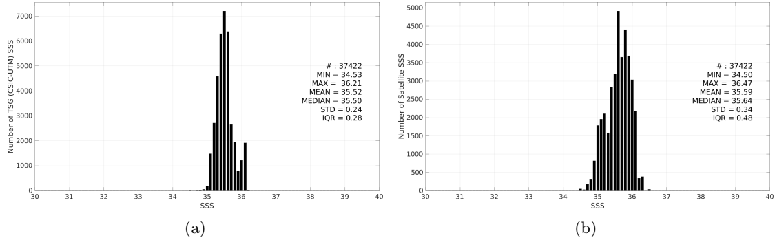
Figure 3: Histograms of SSS from TSG (CSIC-UTM) (a) and SMOS SSS L3 v2 - 9-Days (BEC) (b) considering all match-up pairs per bins of 0.1 over the Indian Ocean Pi-MEP region and for the full satellite product period.
