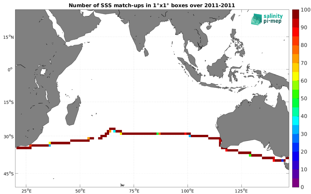
Figure 5: Number of SSS match-ups between TSG (CSIC-UTM) SSS and the SMOS SSS L3 v2 - 9-Days (BEC) SSS product for the Indian Ocean Pi-MEP region over 1^\circ \times 1^\circ boxes and for the full satellite product period.
