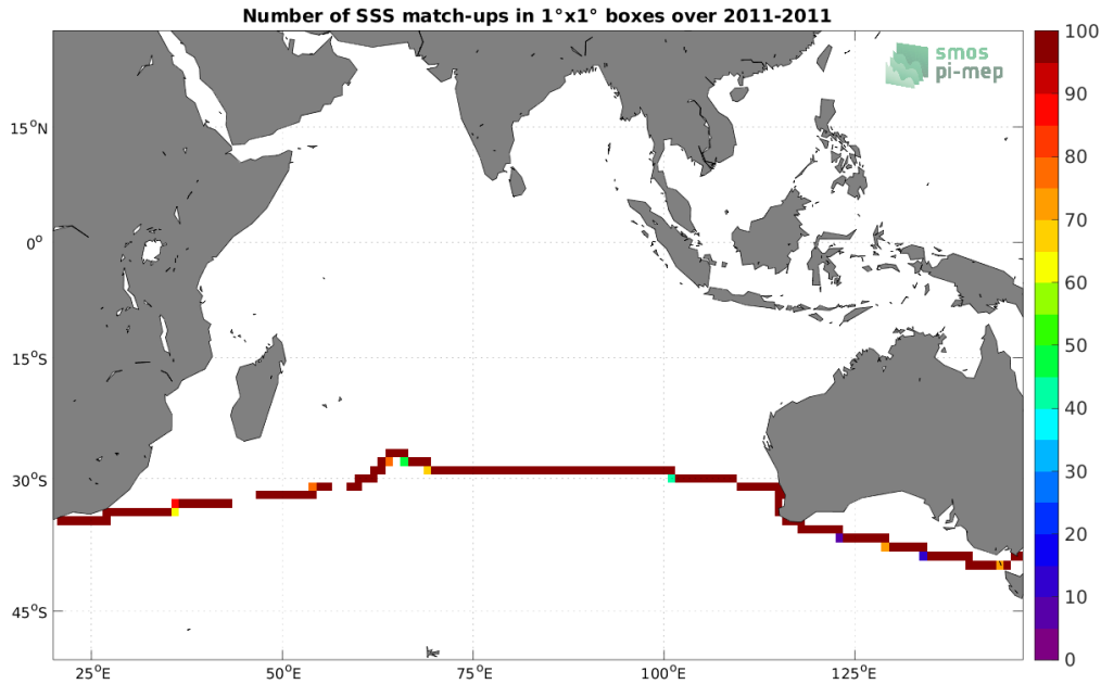
Figure 4: Number of SSS match-ups between TSG (CSIC-UTM) SSS and the SMOS SSS L3 v2 - 9-Days (BEC) SSS product for the Indian Ocean Pi-MEP region over 1^\circ \times 1^\circ boxes and for the full satellite product period.
