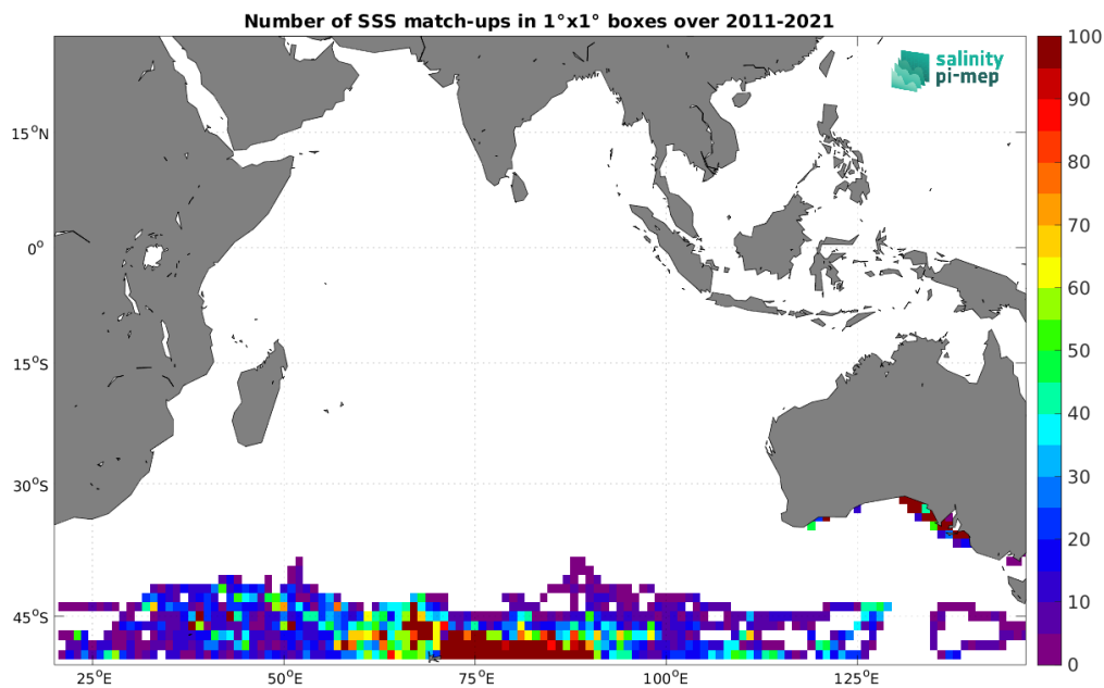
Figure 5: Number of SSS match-ups between Marine mammals SSS and the SMOS SSS L3 v2 - 9-Days (BEC) SSS product for the Indian Ocean Pi-MEP region over 1^\circ \times 1^\circ boxes and for the full satellite product period.
