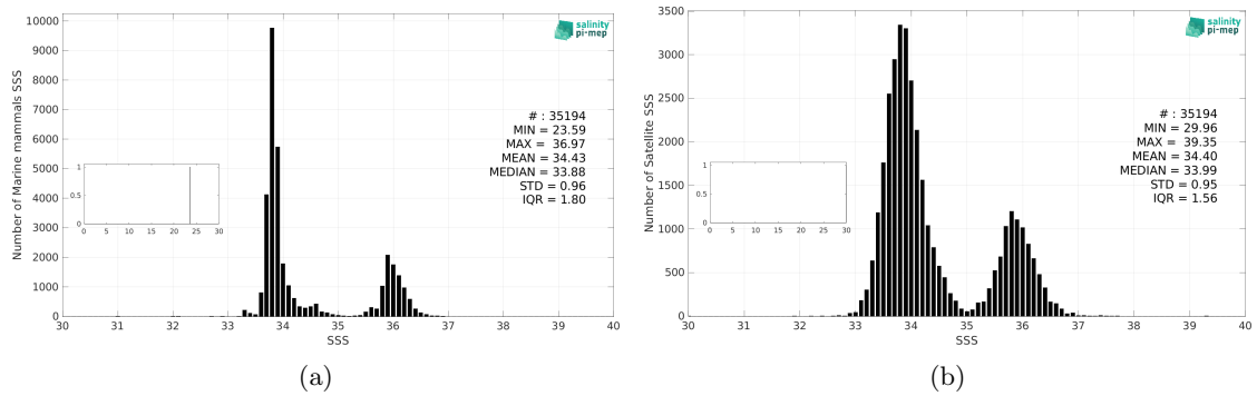
Figure 3: Histograms of SSS from Marine mammals (a) and SMOS SSS L3 v2 - 9-Days (BEC) (b) considering all match-up pairs per bins of 0.1 over the Indian Ocean Pi-MEP region and for the full satellite product period.
