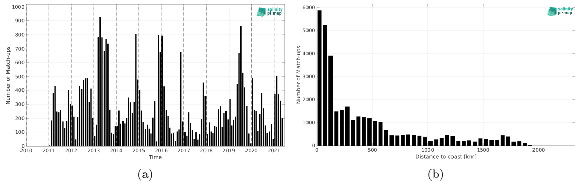
Figure 2: Number of match-ups between Marine mammals and SMOS SSS L3 v2 - 9-Days (BEC) SSS as a function of time (a) and as function of the distance to coast (b) over the Indian Ocean Pi-MEP region and for the full satellite product period.
