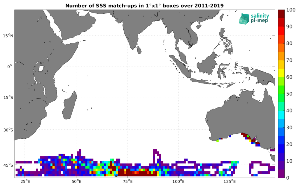
Figure 4: Number of SSS match-ups between Marine mammals SSS and the SMOS SSS L3 v2 - 9-Days (BEC) SSS product for the Indian Ocean Pi-MEP region over 1^\circ \times 1^\circ boxes and for the full satellite product period.
