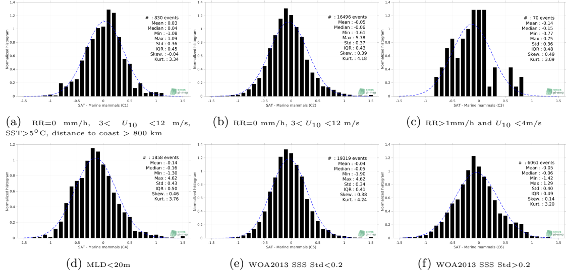
Figure 13: Normalized histogram of \Delta SSS (SMOS SSS L3 v2 - 9-Days (BEC) - Marine mammals) for 6 different subdatasets corresponding to: RR=0 mm/h, 3 < U_{10} < 12 m/s, SST > 5°C, distance to coast > 800 km (a), RR=0 mm/h, 3 < U_{10} < 12 m/s (b), RR > 1mm/h and U_{10} < 4 m/s (c), MLD < 20m (d), WOA2013 SSS Std < 0.2 (e), WOA2013 SSS Std > 0.2 (f).
