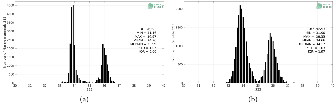
Figure 2: Histograms of SSS from Marine mammals (a) and SMOS SSS L3 v2 - 9-Days (BEC) (b) considering all match-up pairs per bins of 0.1 over the Indian Ocean Pi-MEP region and for the full satellite product period.
