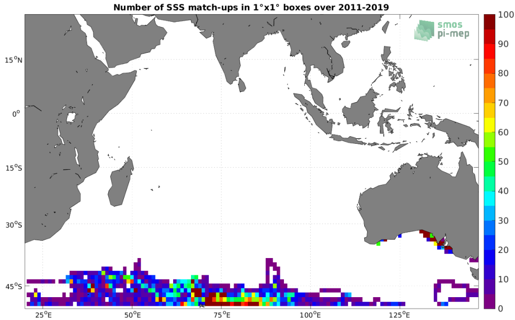
Figure 4: Number of SSS match-ups between Marine mammals SSS and the SMOS SSS L3 v2 - 9-Days (BEC) SSS product for the Indian Ocean Pi-MEP region over 1^\circ \times 1^\circ boxes and for the full satellite product period.
