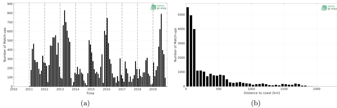
Figure 1: Number of match-ups between Marine mammals and SMOS SSS L3 v2 - 9-Days (BEC) SSS as a function of time (a) and as function of the distance to coast (b) over the Indian Ocean Pi-MEP region and for the full satellite product period.
