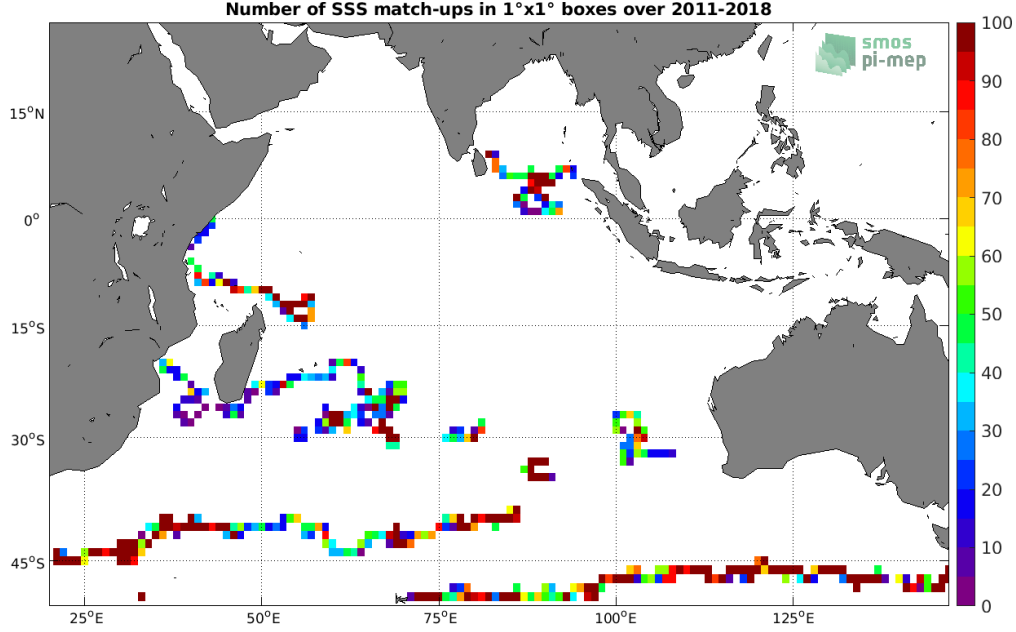
Figure 3: Number of SSS match-ups between Surface drifters SSS and the SMOS SSS L3 v2 - 9-Days (BEC) SSS product for the Indian Ocean Pi-MEP region over 1^\circ \times 1^\circ boxes and for the full satellite product period.
