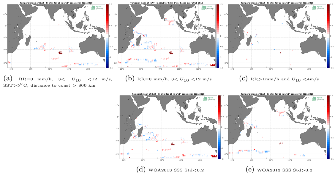
Figure 11: Temporal mean gridded over spatial boxes of size 1^\circ \times 1^\circ of \Delta SSS (SMOS L3 v2 - 9-Days (BEC) - Surface drifters) for 5 different subdatasets corresponding to: RR=0 mm/h, 3 < U_{10} < 12 m/s, SST > 5^\circ C , distance to coast > 800 km (a), RR=0 mm/h, 3 < U_{10} < 12 m/s (b), RR > 1 mm/h and U_{10} < 4 m/s (c), WOA2013 SSS Std < 0.2 (d), WOA2013 SSS Std > 0.2 (e).
