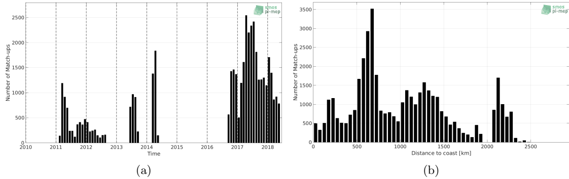
Figure 1: Number of match-ups between Surface drifters and SMOS L3 v2 - 9-Days (BEC) SSS as a function of time (a) and as function of the distance to coast (b) over the Indian Ocean Pi-MEP region and for the full satellite product period.
