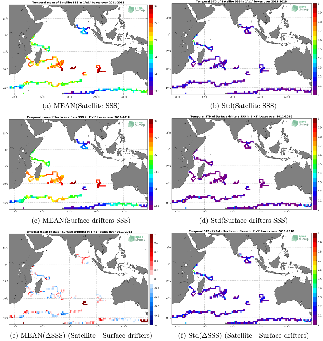
Figure 5: Temporal mean (left) and Std (right) of SSS from SMOS L3 v2 - 9-Days (BEC) (top), Surface drifters (middle), and of \Delta SSS (Satellite - Surface drifters). Only match-up pairs are used to generate these maps.
