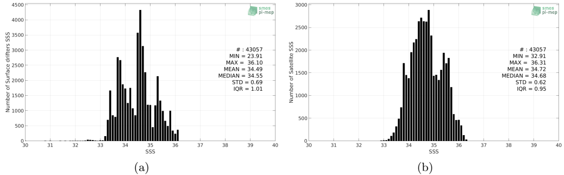
Figure 2: Histograms of SSS from Surface drifters (a) and SMOS L3 v2 - 9-Days (BEC) (b) considering all match-up pairs per bins of 0.1 over the Indian Ocean Pi-MEP region and for the full satellite product period.
