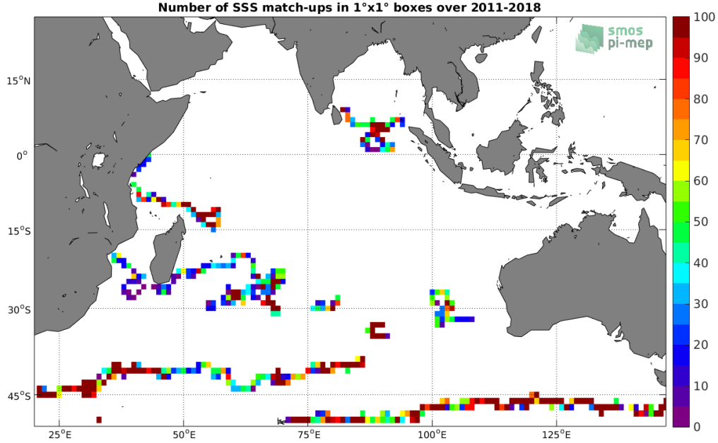
Figure 3: Number of SSS match-ups between Surface drifters SSS and the SMOS L3 v2 - 9-Days (BEC) SSS product for the Indian Ocean Pi-MEP region over 1^\circ \times 1^\circ boxes and for the full satellite product period.
