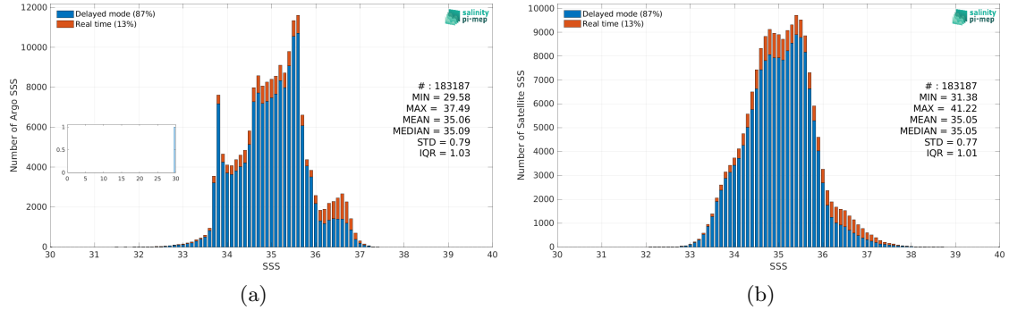
Figure 2: Histograms of SSS from Argo (a) and SMOS SSS L3 v2 - 9-Days (BEC) (b) considering all match-up pairs per bins of 0.1 over the Indian Ocean Pi-MEP region and for the full satellite product period.
