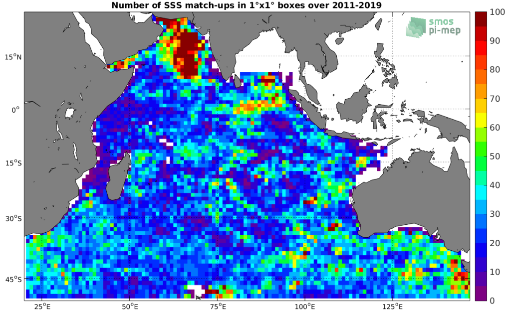
Figure 4: Number of SSS match-ups between Argo SSS and the SMOS SSS L3 v2 - 9-Days (BEC) SSS product for the Indian Ocean Pi-MEP region over 1^\circ \times 1^\circ boxes and for the full satellite product period.
