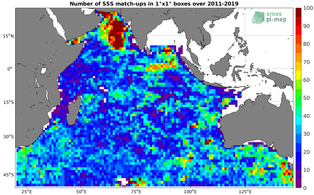
Figure 4: Number of SSS match-ups between Argo SSS and the SMOS SSS L3 v2 - 9-Days (BEC) SSS product for the Indian Ocean Pi-MEP region over 1^\circ \times 1^\circ boxes and for the full satellite product period.
