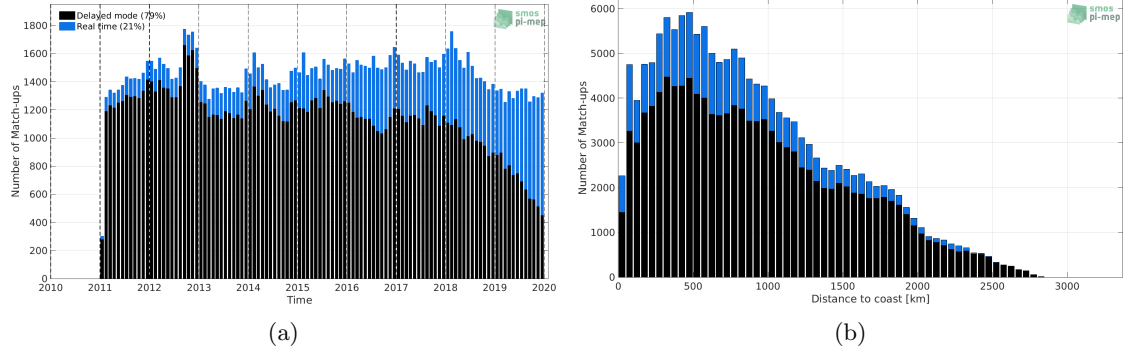
Figure 1: Number of match-ups between Argo and SMOS SSS L3 v2 - 9-Days (BEC) SSS as a function of time (a) and as function of the distance to coast (b) over the Indian Ocean Pi-MEP region and for the full satellite product period.
