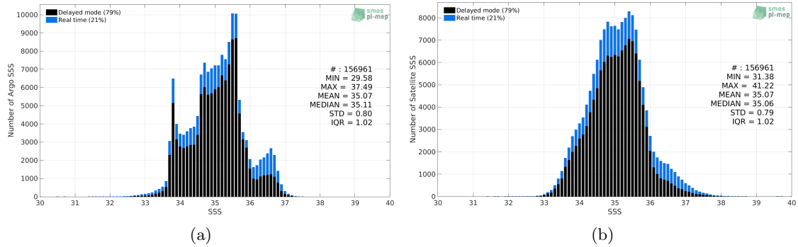
Figure 2: Histograms of SSS from Argo (a) and SMOS SSS L3 v2 - 9-Days (BEC) (b) considering all match-up pairs per bins of 0.1 over the Indian Ocean Pi-MEP region and for the full satellite product period.
