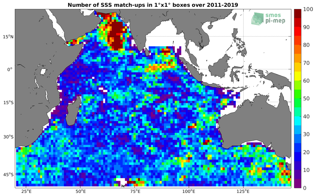
Figure 4: Number of SSS match-ups between Argo SSS and the SMOS SSS L3 v2 - 9-Days (BEC) SSS product for the Indian Ocean Pi-MEP region over 1°x1° boxes and for the full satellite product period.
