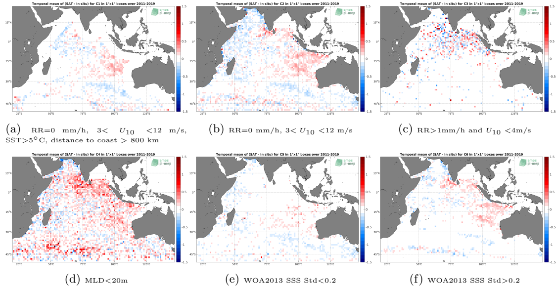
Figure 12: Temporal mean gridded over spatial boxes of size 1^\circ \times 1^\circ of \Delta SSS (SMOS SSS L3 v2 - 9-Days (BEC) - Argo) for 6 different subdatasets corresponding to: RR=0 mm/h, 3 < U_{10} < 12 m/s, SST > 5^\circ C , distance to coast > 800 km (a), RR=0 mm/h, 3 < U_{10} < 12 m/s (b), RR > 1 mm/h and U_{10} < 4 m/s (c), MLD < 20 m (d), WOA2013 SSS Std < 0.2 (e), WOA2013 SSS Std > 0.2 (f).
