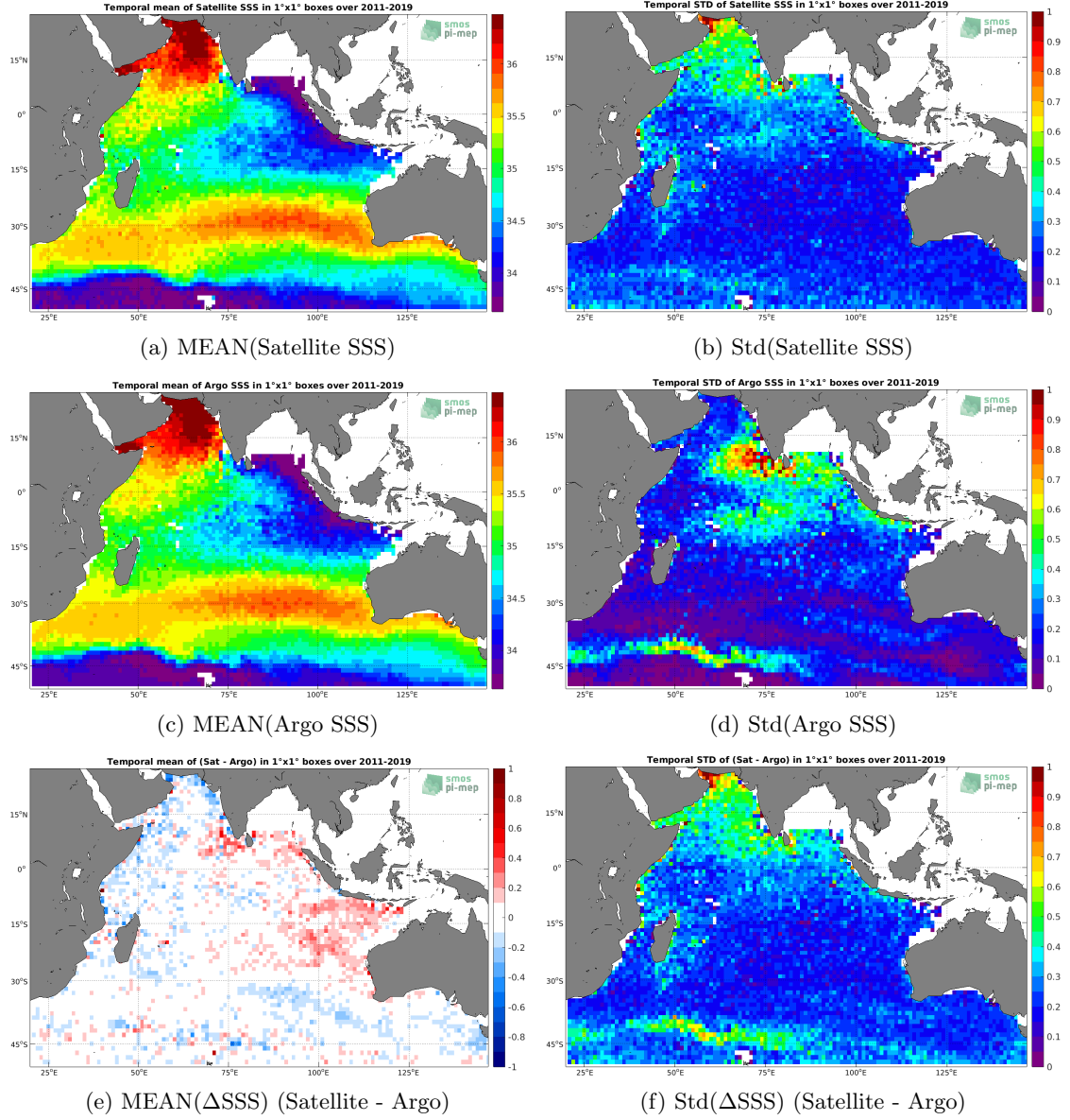
Figure 6: Temporal mean (left) and Std (right) of SSS from SMOS SSS L3 v2 - 9-Days (BEC) (top), Argo (middle), and of \Delta SSS (Satellite - Argo). Only match-up pairs are used to generate these maps.
