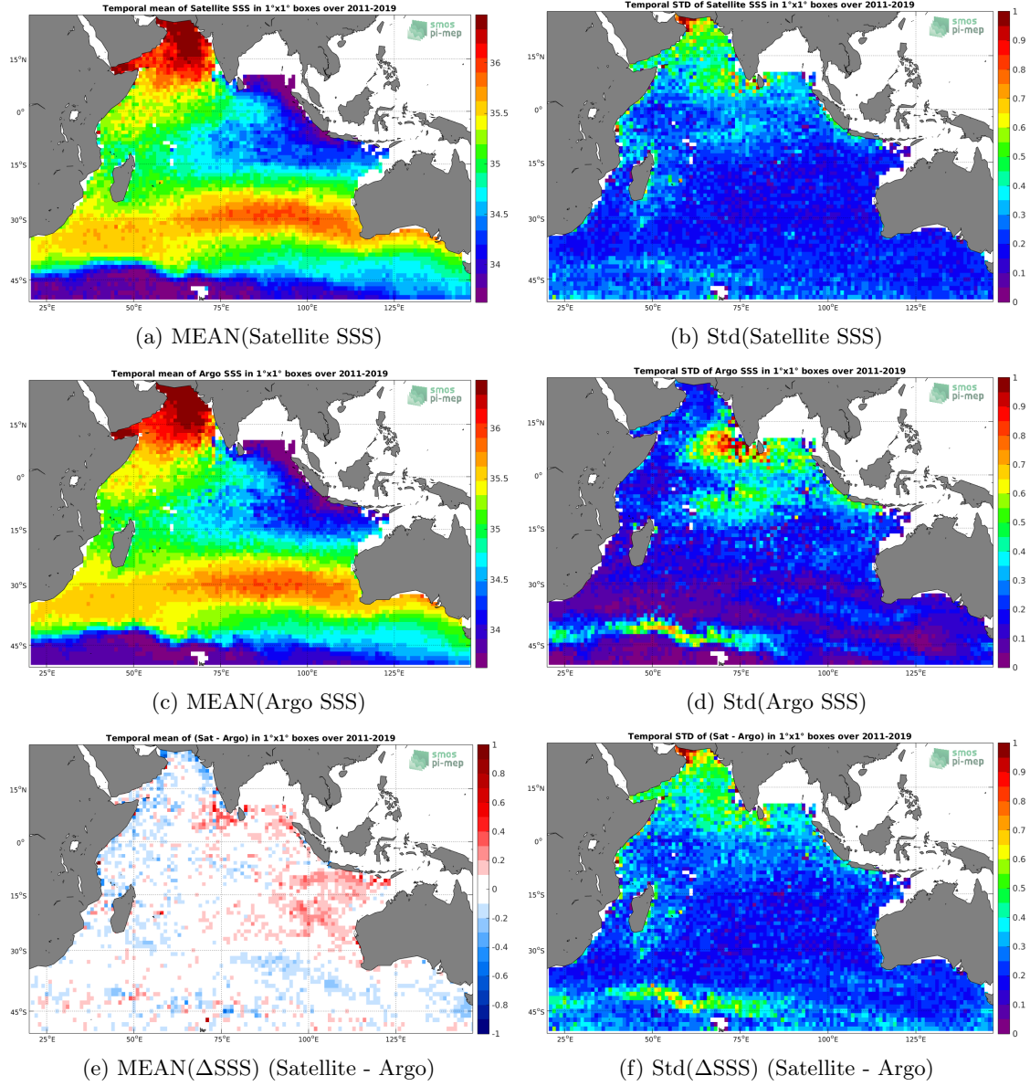
Figure 6: Temporal mean (left) and Std (right) of SSS from SMOS L3 v2 - 9-Days (BEC) (top), Argo (middle), and of \Delta SSS (Satellite - Argo). Only match-up pairs are used to generate these maps.
