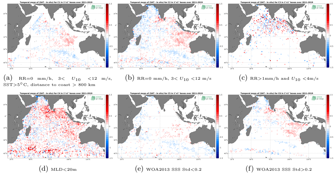
Figure 12: Temporal mean gridded over spatial boxes of size 1^\circ \times 1^\circ of \Delta SSS (SMOS L3 v2 - 9-Days (BEC) - Argo) for 6 different subdatasets corresponding to: RR=0 mm/h, 3 < U_{10} < 12 m/s, SST > 5^\circ C , distance to coast > 800 km (a), RR=0 mm/h, 3 < U_{10} < 12 m/s (b), RR > 1 mm/h and U_{10} < 4 m/s (c), MLD < 20 m (d), WOA2013 SSS Std < 0.2 (e), WOA2013 SSS Std > 0.2 (f).
