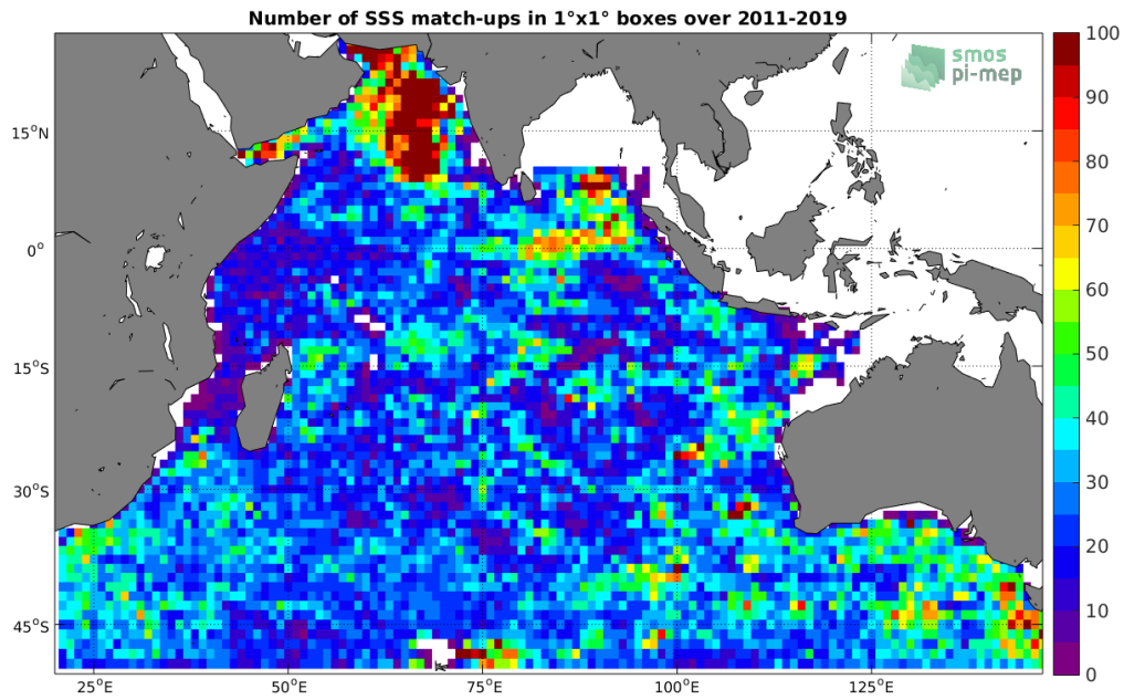
Figure 4: Number of SSS match-ups between Argo SSS and the SMOS L3 v2 - 9-Days (BEC) SSS product for the Indian Ocean Pi-MEP region over 1°x1° boxes and for the full satellite product period.
