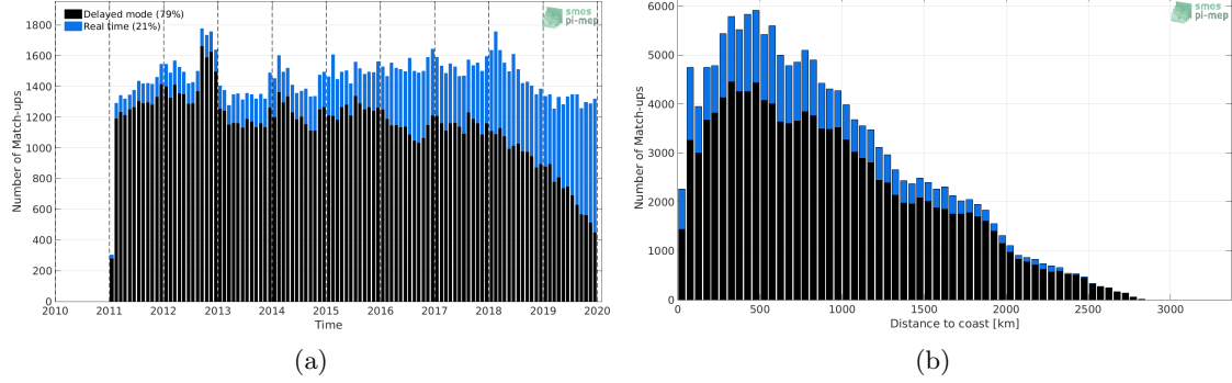
Figure 1: Number of match-ups between Argo and SMOS L3 v2 - 9-Days (BEC) SSS as a function of time (a) and as function of the distance to coast (b) over the Indian Ocean Pi-MEP region and for the full satellite product period.
