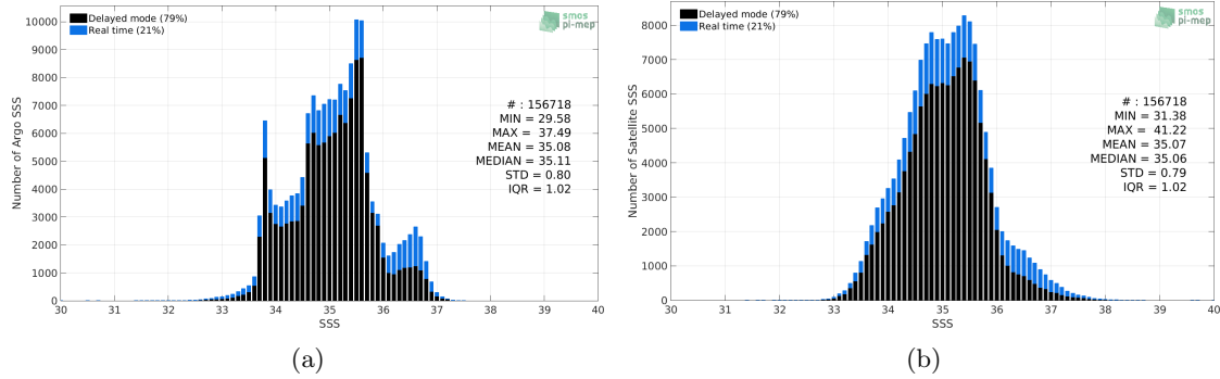
Figure 2: Histograms of SSS from Argo (a) and SMOS L3 v2 - 9-Days (BEC) (b) considering all match-up pairs per bins of 0.1 over the Indian Ocean Pi-MEP region and for the full satellite product period.
