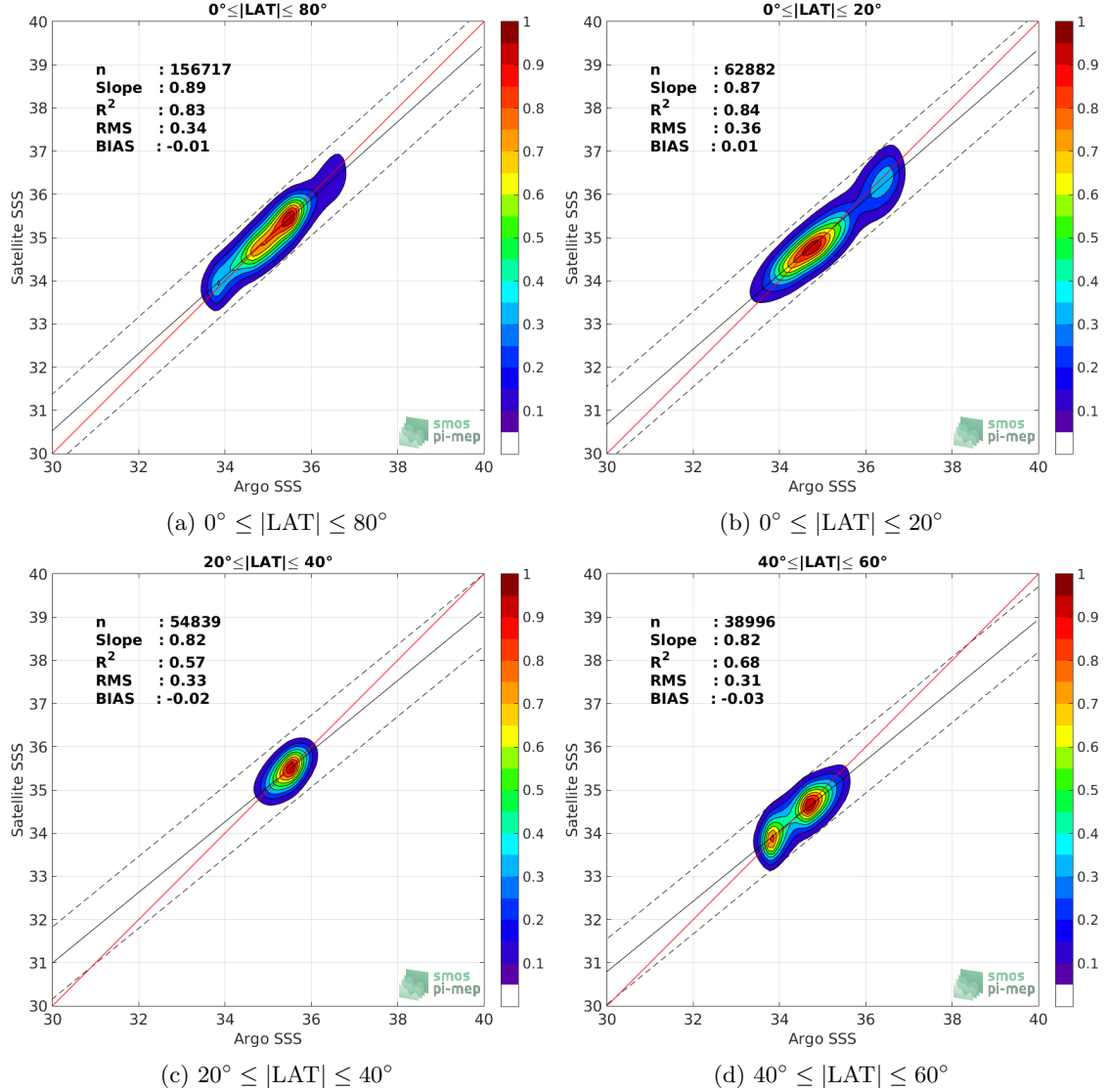
Figure 9: Contour maps of the concentration of SMOS L3 v2 - 9-Days (BEC) SSS (y-axis) versus Argo SSS (x-axis) at match-up pairs for different latitude bands. For each plot, the red line shows x=y . The black thin and dashed lines indicate a linear fit through the data cloud and the \pm 95\% confidence levels, respectively. The number match-up pairs n , the slope and R^2 coefficient of the linear fit, the root mean square (RMS) and the mean bias between satellite and in situ data are indicated for each latitude band in each plots.
