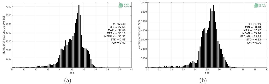
Figure 2: Histograms of SSS from TSG-LEGOS-DM (a) and SMOS-L3-BEC-OA-V1-9DAYS-0.25DEG (b) considering all match-up pairs per bins of 0.1 over the Indian Ocean Pi-MEP region and for the full satellite product period.
