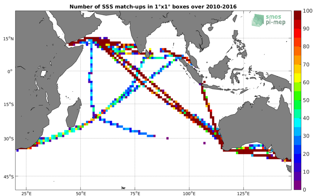
Figure 4: Number of SSS match-ups between TSG-LEGOS-DM SSS and the SMOS-L3-BEC-OA-V1-9DAYS-0.25DEG SSS product for the Indian Ocean Pi-MEP region over 1^\circ \times 1^\circ boxes and for the full satellite product period.
