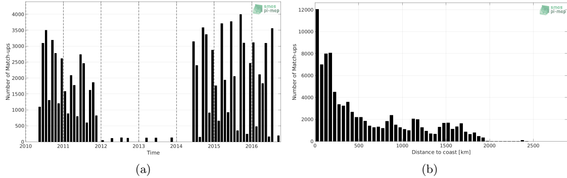
Figure 1: Number of match-ups between TSG-LEGOS-DM and SMOS-L3-BEC-OA-V1-9DAYS-0.25DEG SSS as a function of time (a) and as function of the distance to coast (b) over the Indian Ocean Pi-MEP region and for the full satellite product period.
