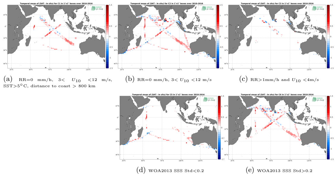
Figure 12: Temporal mean gridded over spatial boxes of size 1^\circ \times 1^\circ of \Delta SSS (SMOS-L3-BEC-OA-V1-9DAYS-0.25DEG - TSG-LEGOS-DM) for 5 different subdatasets corresponding to:RR=0 mm/h, 3 < U_{10} < 12 m/s, SST > 5^\circ\text{C} , distance to coast > 800 km (a), RR=0 mm/h, 3 < U_{10} < 12 m/s (b), RR > 1 mm/h and U_{10} < 4 m/s (c), WOA2013 SSS Std < 0.2 (d), WOA2013 SSS Std > 0.2 (e).
