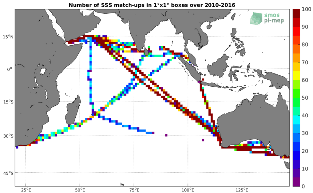
Figure 4: Number of SSS match-ups between TSG-LEGOS-DM SSS and the SMOS-L3-BEC-OA-V1-9DAYS-0.25DEG SSS product for the Indian Ocean Pi-MEP region over 1^\circ \times 1^\circ boxes and for the full satellite product period.
