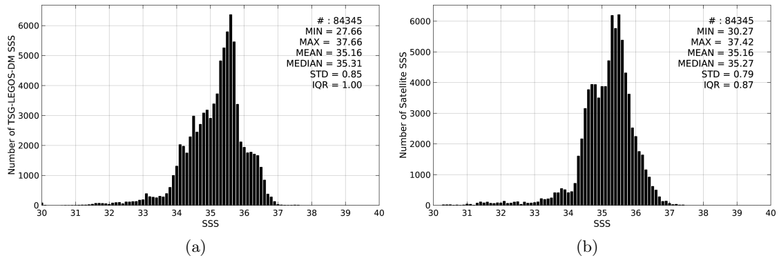
Figure 2: Histograms of SSS from TSG-LEGOS-DM (a) and SMOS-L3-BEC-OA-V1-9DAYS-0.25DEG (b) considering all match-up pairs per bins of 0.1 over the Indian Ocean Pi-MEP region and for the full satellite product period.
