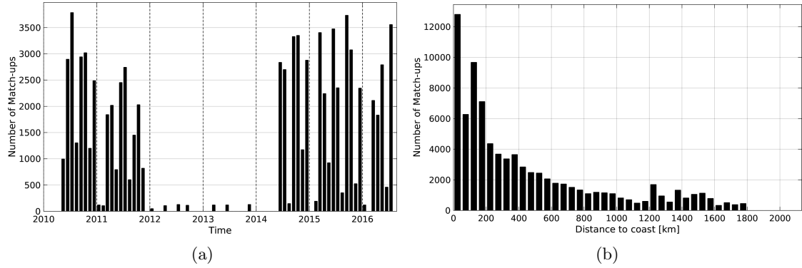
Figure 1: Number of match-ups between TSG-LEGOS-DM and SMOS-L3-BEC-OA-V1-9DAYS-0.25DEG SSS as a function of time (a) and as function of the distance to coast (b) over the Indian Ocean Pi-MEP region and for the full satellite product period.
