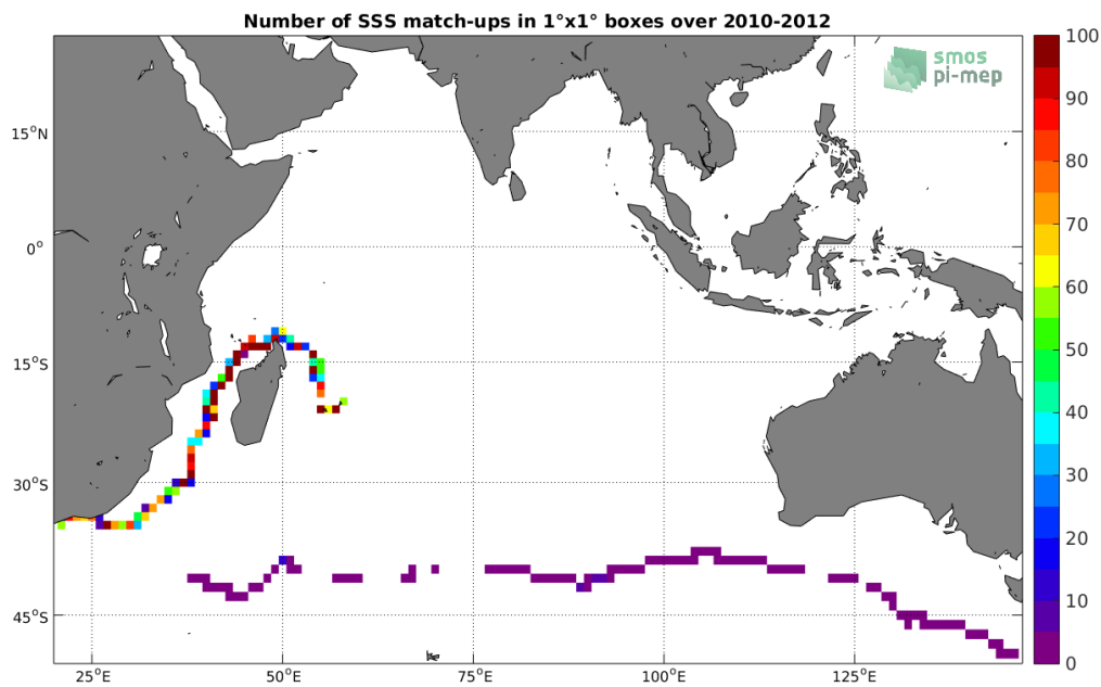
Figure 4: Number of SSS match-ups between TSG-GOSUD-Sailing-ship SSS and the SMOS-L3-BEC-OA-V1-9DAYS-0.25DEG SSS product for the Indian Ocean Pi-MEP region over 1°x1° boxes and for the full satellite product period.
