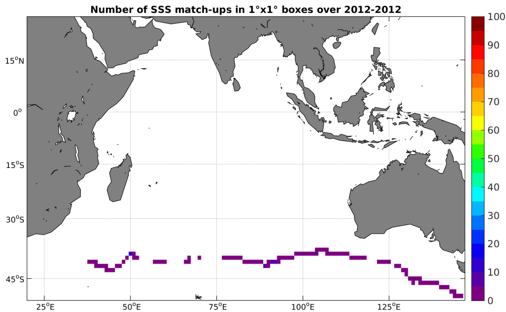
Figure 4: Number of SSS match-ups between TSG-GOSUD-Sailing-ship SSS and the SMOS-L3-BEC-OA-V1-9DAYS-0.25DEG SSS product for the Indian Ocean Pi-MEP region over 1^\circ \times 1^\circ boxes and for the full satellite product period.
