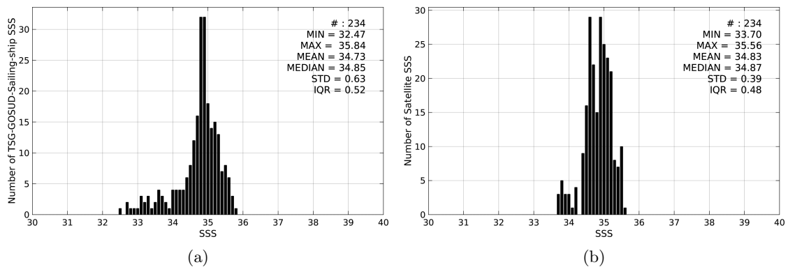
Figure 2: Histograms of SSS from TSG-GOSUD-Sailing-ship (a) and SMOS-L3-BEC-OA-V1-9DAYS-0.25DEG (b) considering all match-up pairs per bins of 0.1 over the Indian Ocean Pi-MEP region and for the full satellite product period.
