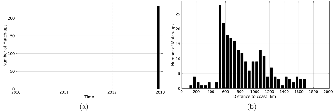
Figure 1: Number of match-ups between TSG-GOSUD-Sailing-ship and SMOS-L3-BEC-OA-V1-9DAYS-0.25DEG SSS as a function of time (a) and as function of the distance to coast (b) over the Indian Ocean Pi-MEP region and for the full satellite product period.
