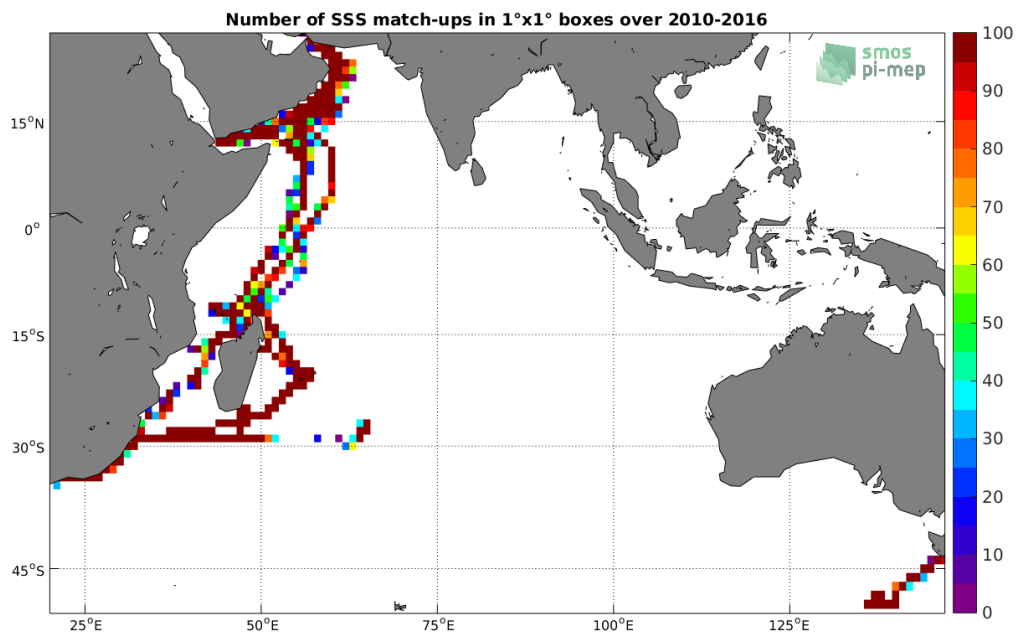
Figure 4: Number of SSS match-ups between TSG-GOSUD-Research-vessel SSS and the SMOS-L3-BEC-OA-V1-9DAYS-0.25DEG SSS product for the Indian Ocean Pi-MEP region over 1^\circ \times 1^\circ boxes and for the full satellite product period.
