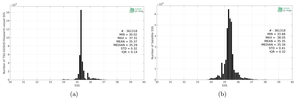
Figure 2: Histograms of SSS from TSG-GOSUD-Research-vessel (a) and SMOS-L3-BEC-OA-V1-9DAYS-0.25DEG (b) considering all match-up pairs per bins of 0.1 over the Indian Ocean Pi-MEP region and for the full satellite product period.
