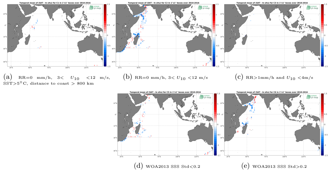
Figure 12: Temporal mean gridded over spatial boxes of size 1^\circ \times 1^\circ of \Delta SSS (SMOS-L3-BEC-OA-V1-9DAYS-0.25DEG - TSG-GOSUD-Research-vessel) for 5 different subdatasets corresponding to:RR=0 mm/h, 3 < U_{10} < 12 m/s, SST >5^\circ C, distance to coast > 800 km (a), RR=0 mm/h, 3 < U_{10} < 12 m/s (b), RR >1 mm/h and U_{10} < 4 m/s (c), WOA2013 SSS Std <0.2 (d), WOA2013 SSS Std >0.2 (e).
