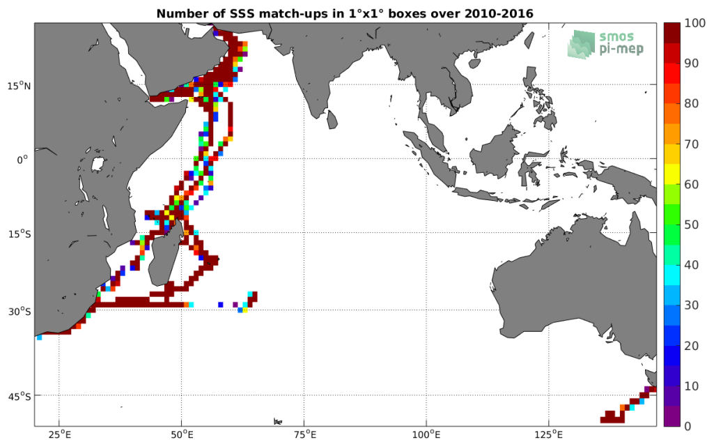
Figure 4: Number of SSS match-ups between TSG-GOSUD-Research-vessel SSS and the SMOS-L3-BEC-OA-V1-9DAYS-0.25DEG SSS product for the Indian Ocean Pi-MEP region over 1^\circ \times 1^\circ boxes and for the full satellite product period.
