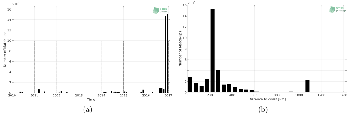
Figure 1: Number of match-ups between TSG-GOSUD-Research-vessel and SMOS-L3-BEC-OA-V1-9DAYS-0.25DEG SSS as a function of time (a) and as function of the distance to coast (b) over the Indian Ocean Pi-MEP region and for the full satellite product period.
