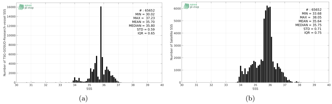
Figure 2: Histograms of SSS from TSG-GOSUD-Research-vessel (a) and SMOS-L3-BEC-OA-V1-9DAYS-0.25DEG (b) considering all match-up pairs per bins of 0.1 over the Indian Ocean Pi-MEP region and for the full satellite product period.
