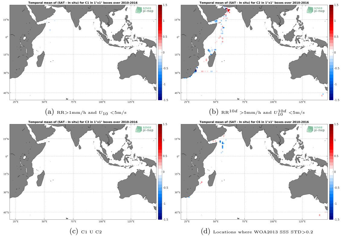
Figure 12: Temporal mean gridded over spatial boxes of size 1^\circ \times 1^\circ of \Delta SSS (SMOS-L3-BEC-OA-V1-9DAYS-0.25DEG - TSG-GOSUD-Research-vessel) for 4 different subdatasets corresponding to: RR > 1mm/h and U_{10} < 5\text{m/s} (a), RR^{10d} > 5\text{mm/h} and U_{10}^{10d} < 5\text{m/s} (b), C1 U C2 (c), Locations where WOA2013 SSS STD > 0.2 (d).
