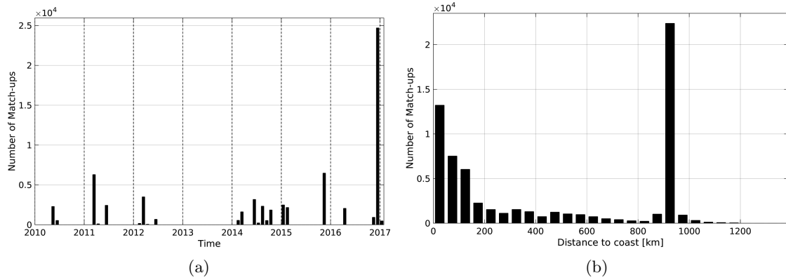
Figure 1: Number of match-ups between TSG-GOSUD-Research-vessel and SMOS-L3-BEC-OA-V1-9DAYS-0.25DEG SSS as a function of time (a) and as function of the distance to coast (b) over the Indian Ocean Pi-MEP region and for the full satellite product period.
