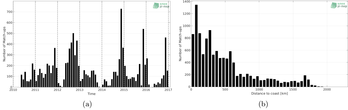
Figure 1: Number of match-ups between Sea mammals and SMOS-L3-BEC-OA-V1-9DAYS-0.25DEG SSS as a function of time (a) and as function of the distance to coast (b) over the Indian Ocean Pi-MEP region and for the full satellite product period.
