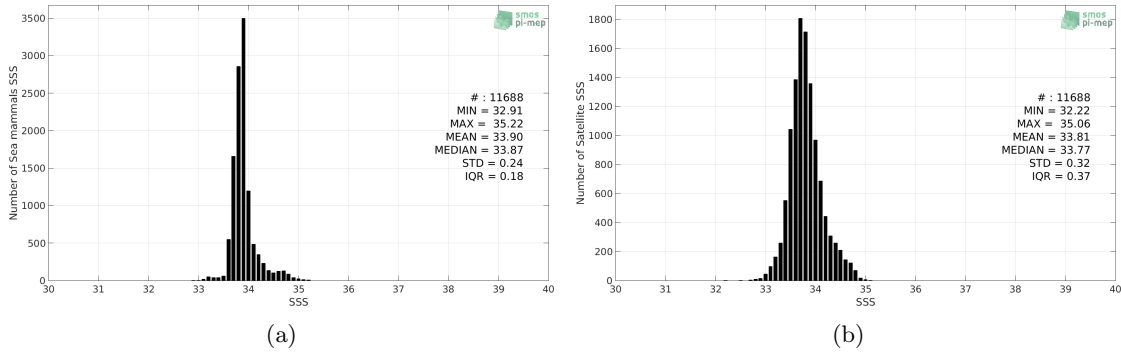
Figure 2: Histograms of SSS from Sea mammals (a) and SMOS-L3-BEC-OA-V1-9DAYS-0.25DEG (b) considering all match-up pairs per bins of 0.1 over the Indian Ocean Pi-MEP region and for the full satellite product period.
