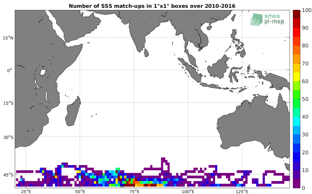
Figure 4: Number of SSS match-ups between Sea mammals SSS and the SMOS-L3-BEC-OA-V1-9DAYS-0.25DEG SSS product for the Indian Ocean Pi-MEP region over 1°x1° boxes and for the full satellite product period.
