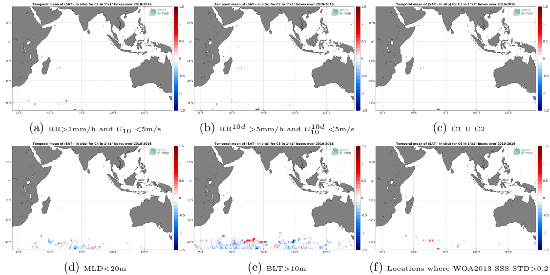
Figure 12: Temporal mean gridded over spatial boxes of size 1^\circ \times 1^\circ of \Delta\text{SSS} (SMOS-L3-BEC-OA-V1-9DAYS-0.25DEG - Sea mammals) for 6 different subdatasets corresponding to: \text{RR} > 1\text{mm/h} and U_{10} < 5\text{m/s} (a), \text{RR}^{10d} > 5\text{mm/h} and U_{10}^{10d} < 5\text{m/s} (b), C1 U C2 (c), \text{MLD} < 20\text{m} (d), \text{BLT} > 10\text{m} (e), Locations where WOA2013 SSS STD > 0.2 (f).
