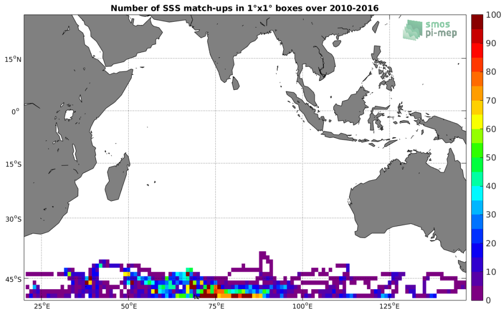
Figure 4: Number of SSS match-ups between Sea mammals SSS and the SMOS-L3-BEC-OA-V1-9DAYS-0.25DEG SSS product for the Indian Ocean Pi-MEP region over 1^\circ \times 1^\circ boxes and for the full satellite product period.
