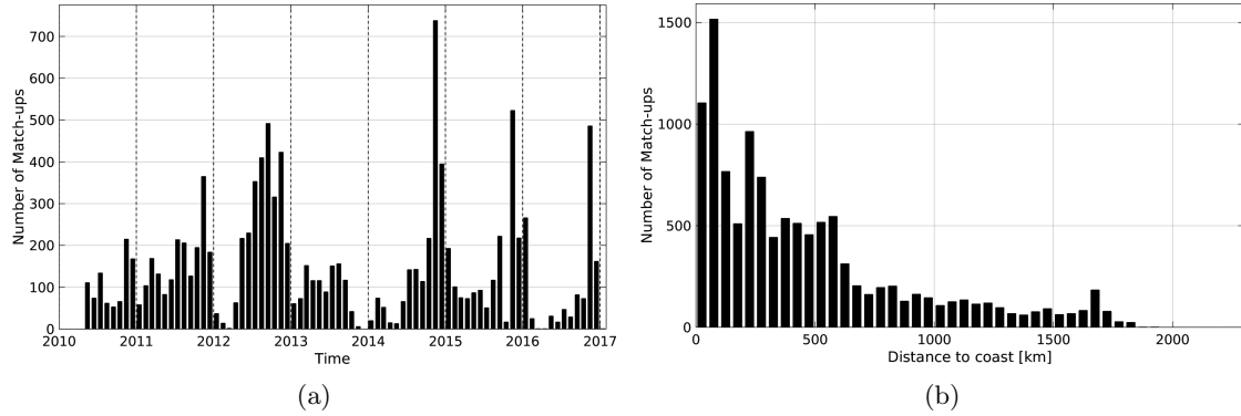
Figure 1: Number of match-ups between Sea mammals and SMOS-L3-BEC-OA-V1-9DAYS-0.25DEG SSS as a function of time (a) and as function of the distance to coast (b) over the Indian Ocean Pi-MEP region and for the full satellite product period.
