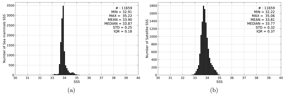
Figure 2: Histograms of SSS from Sea mammals (a) and SMOS-L3-BEC-OA-V1-9DAYS-0.25DEG (b) considering all match-up pairs per bins of 0.1 over the Indian Ocean Pi-MEP region and for the full satellite product period.
