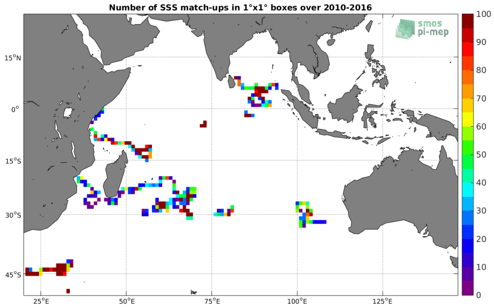
Figure 3: Number of SSS match-ups between Surface drifters SSS and the SMOS-L3-BEC-OA-V1-9DAYS-0.25DEG SSS product for the Indian Ocean Pi-MEP region over 1°x1° boxes and for the full satellite product period.
