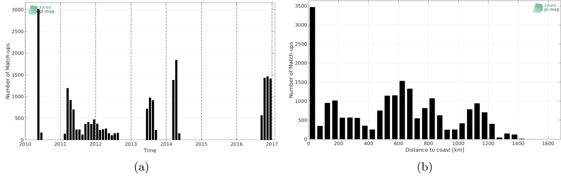
Figure 1: Number of match-ups between Surface drifters and SMOS-L3-BEC-OA-V1-9DAYS-0.25DEG SSS as a function of time (a) and as function of the distance to coast (b) over the Indian Ocean Pi-MEP region and for the full satellite product period.
