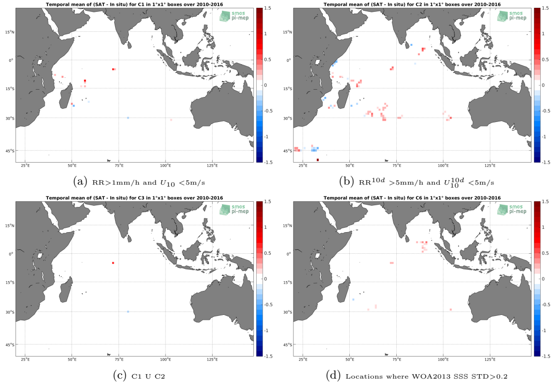
Figure 11: Temporal mean gridded over spatial boxes of size 1^\circ \times 1^\circ of \Delta SSS (SMOS-L3-BEC-OA-V1-9DAYS-0.25DEG - Surface drifters) for 4 different subdatasets corresponding to: RR > 1\text{mm/h} and U_{10} < 5\text{m/s} (a), RR^{10d} > 5\text{mm/h} and U_{10}^{10d} < 5\text{m/s} (b), C1 U C2 (c), Locations where WOA2013 SSS STD > 0.2 (d).
