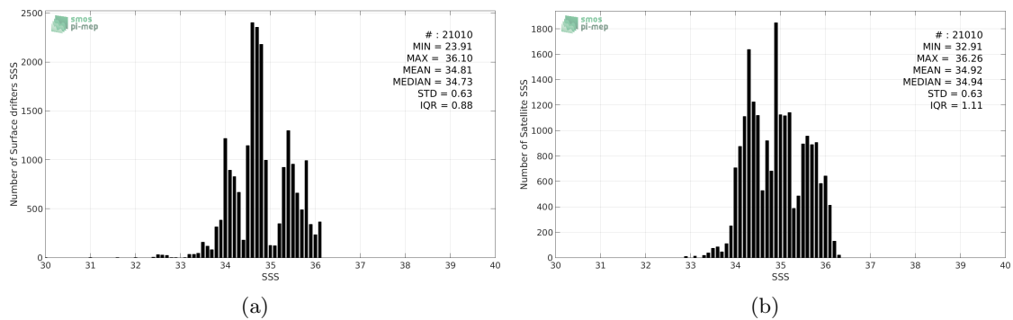
Figure 2: Histograms of SSS from Surface drifters (a) and SMOS-L3-BEC-OA-V1-9DAYS-0.25DEG (b) considering all match-up pairs per bins of 0.1 over the Indian Ocean Pi-MEP region and for the full satellite product period.
