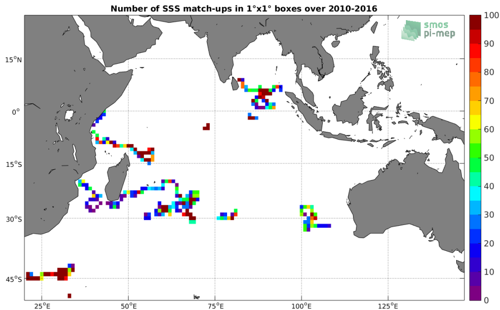
Figure 3: Number of SSS match-ups between Surface drifters SSS and the SMOS-L3-BEC-OA-V1-9DAYS-0.25DEG SSS product for the Indian Ocean Pi-MEP region over 1^\circ \times 1^\circ boxes and for the full satellite product period.
