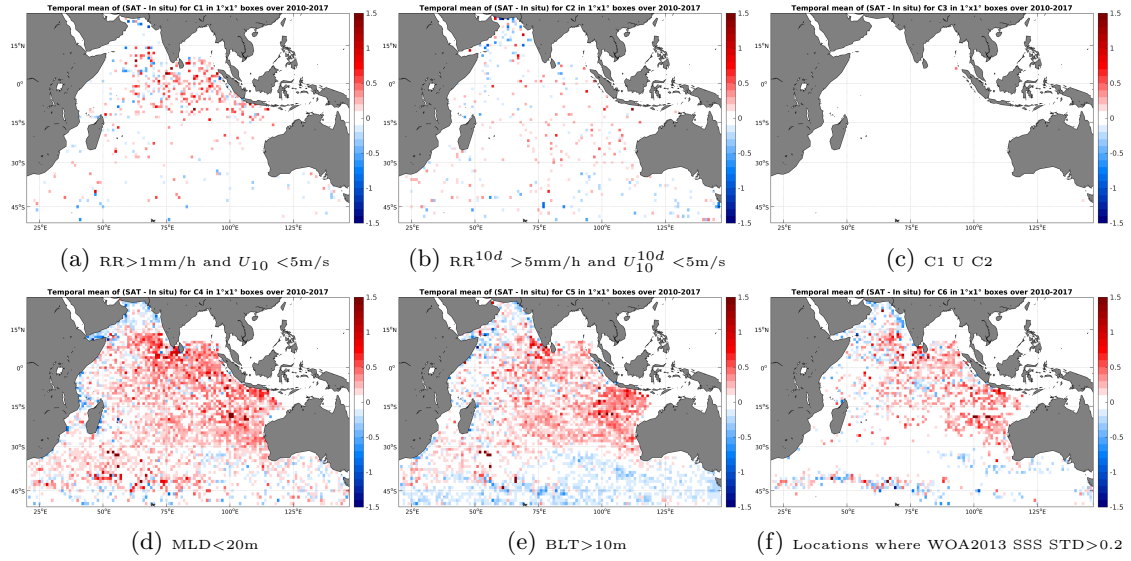
Figure 12: Temporal mean gridded over spatial boxes of size 1^\circ \times 1^\circ of \Delta SSS (SMOS-L3-BEC-OA-V1-9DAYS-0.25DEG - Argo) for 6 different subdatasets corresponding to: RR > 1\text{mm/h} and U_{10} < 5\text{m/s} (a), RR^{10d} > 5\text{mm/h} and U_{10}^{10d} < 5\text{m/s} (b), C1 U C2 (c), MLD < 20\text{m} (d), BLT > 10\text{m} (e), Locations where WOA2013 SSS STD > 0.2 (f).
