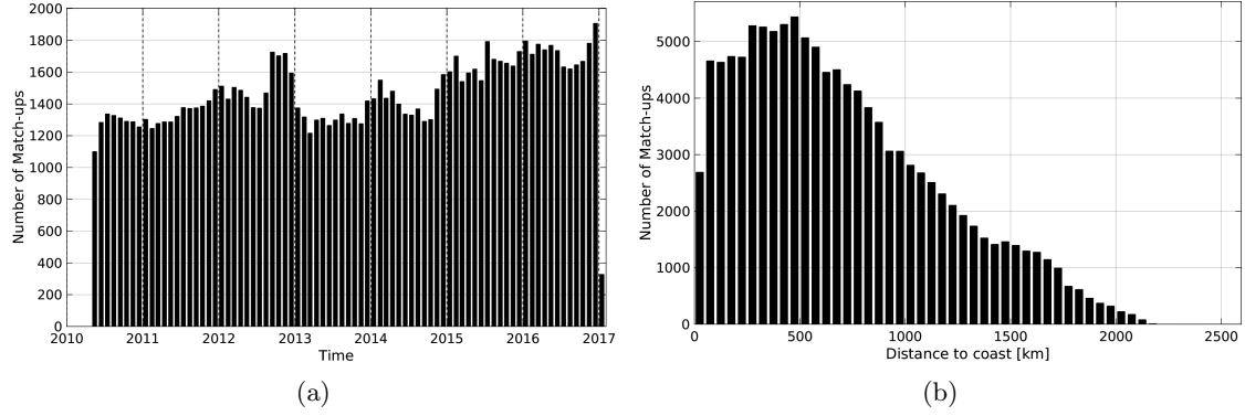
Figure 1: Number of match-ups between Argo and SMOS-L3-BEC-OA-V1-9DAYS-0.25DEG SSS as a function of time (a) and as function of the distance to coast (b) over the Indian Ocean Pi-MEP region and for the full satellite product period.
