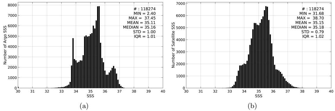
Figure 2: Histograms of SSS from Argo (a) and SMOS-L3-BEC-OA-V1-9DAYS-0.25DEG (b) considering all match-up pairs per bins of 0.1 over the Indian Ocean Pi-MEP region and for the full satellite product period.
