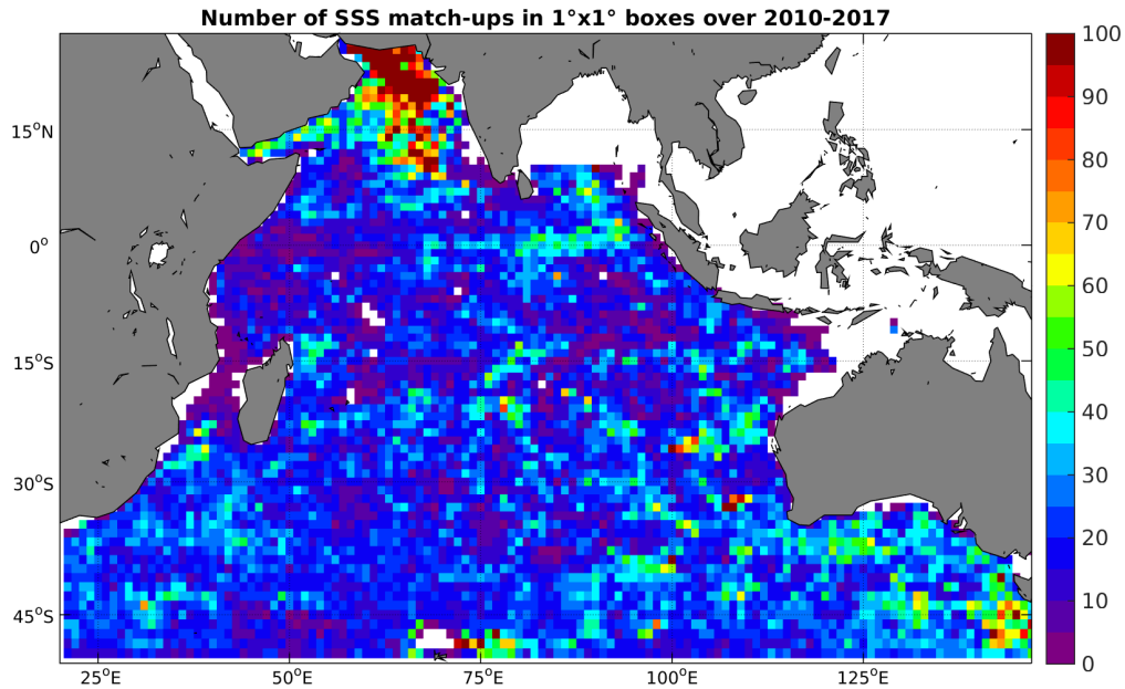
Figure 4: Number of SSS match-ups between Argo SSS and the SMOS-L3-BEC-OA-V1-9DAYS-0.25DEG SSS product for the Indian Ocean Pi-MEP region over 1^\circ \times 1^\circ boxes and for the full satellite product period.
