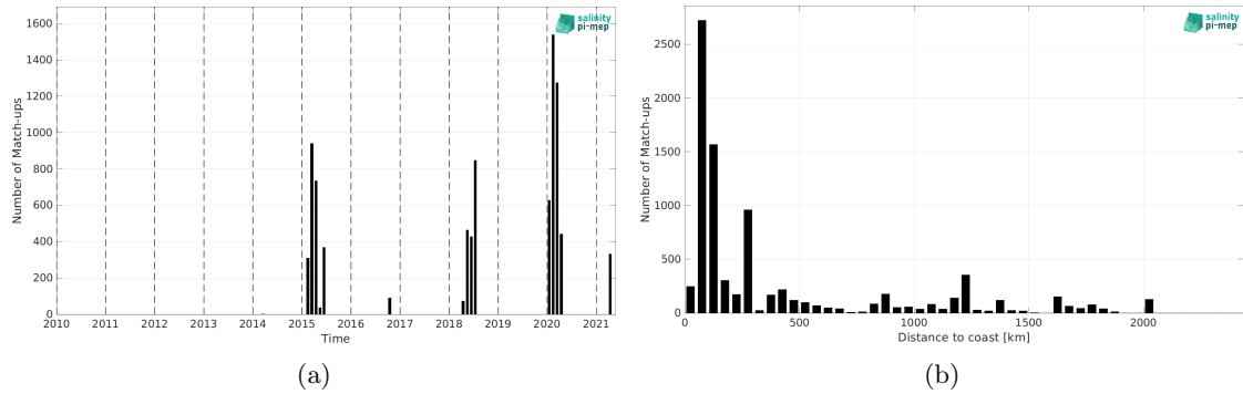
Figure 1: Number of match-ups between TSG (SAMOS) and SMOS SSS L2 v700 (ESA) SSS as a function of time (a) and as function of the distance to coast (b) over the Indian Ocean Pi-MEP region and for the full satellite product period.
