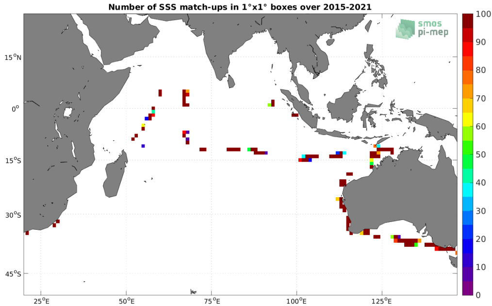
Figure 4: Number of SSS match-ups between TSG (SAMOS) SSS and the SMOS SSS L2 v700 (ESA) SSS product for the Indian Ocean Pi-MEP region over 1^\circ \times 1^\circ boxes and for the full satellite product period.
