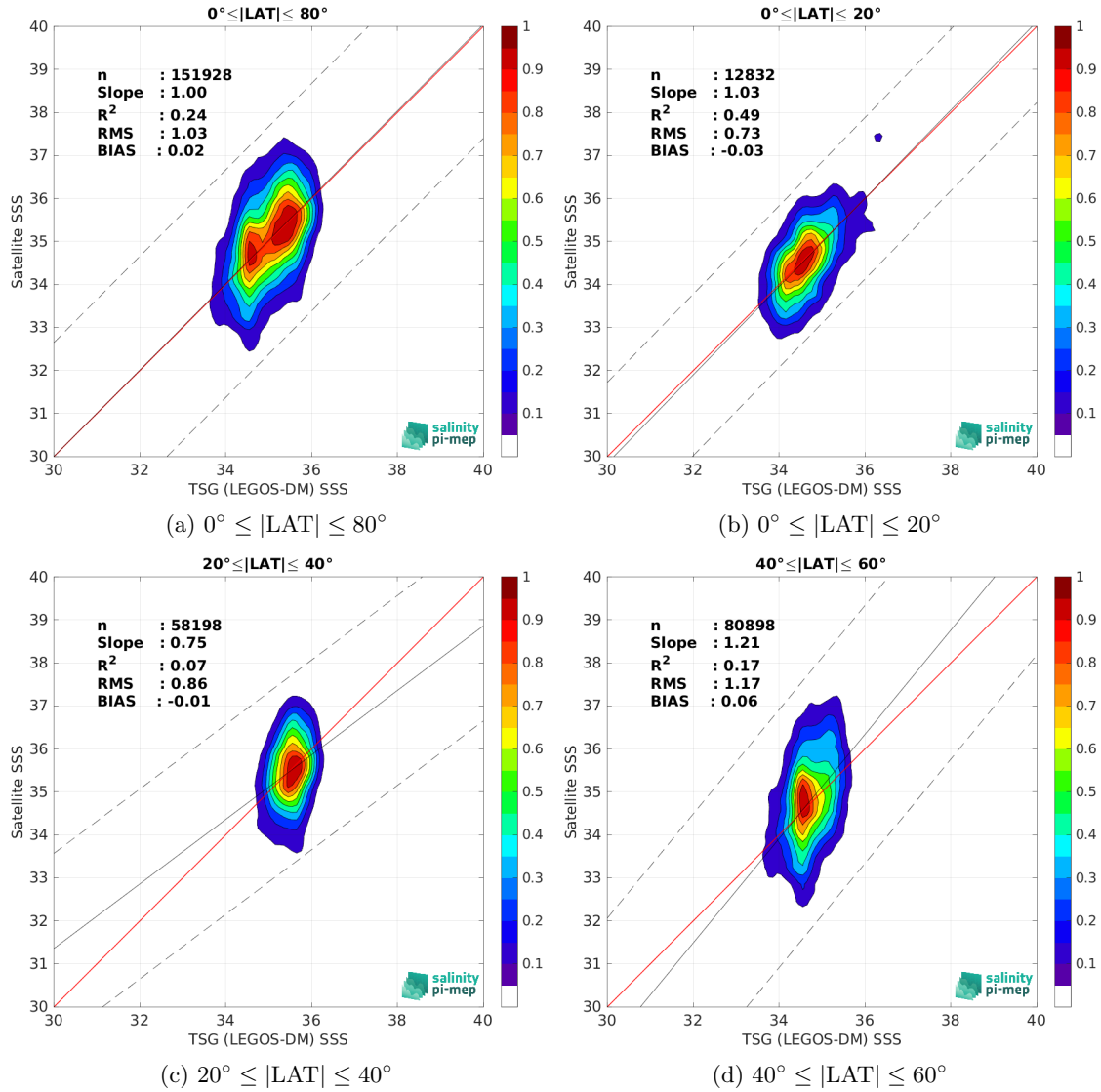
Figure 10: Contour maps of the concentration of SMOS SSS L2 v700 (ESA) SSS (y-axis) versus TSG (LEGOS-DM) SSS (x-axis) at match-up pairs for different latitude bands. For each plot, the red line shows x=y . The black thin and dashed lines indicate a linear fit through the data cloud and the \pm 95\% confidence levels, respectively. The number match-up pairs n , the slope and R^2 coefficient of the linear fit, the root mean square (RMS) and the mean bias between satellite and in situ data are indicated for each latitude band in each plots.
