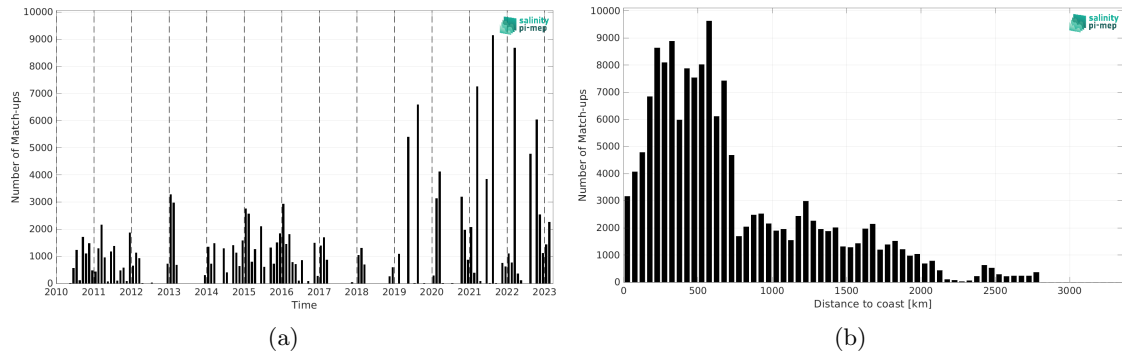
Figure 2: Number of match-ups between TSG (LEGOS-DM) and SMOS SSS L2 v700 (ESA) SSS as a function of time (a) and as function of the distance to coast (b) over the Indian Ocean Pi-MEP region and for the full satellite product period.
