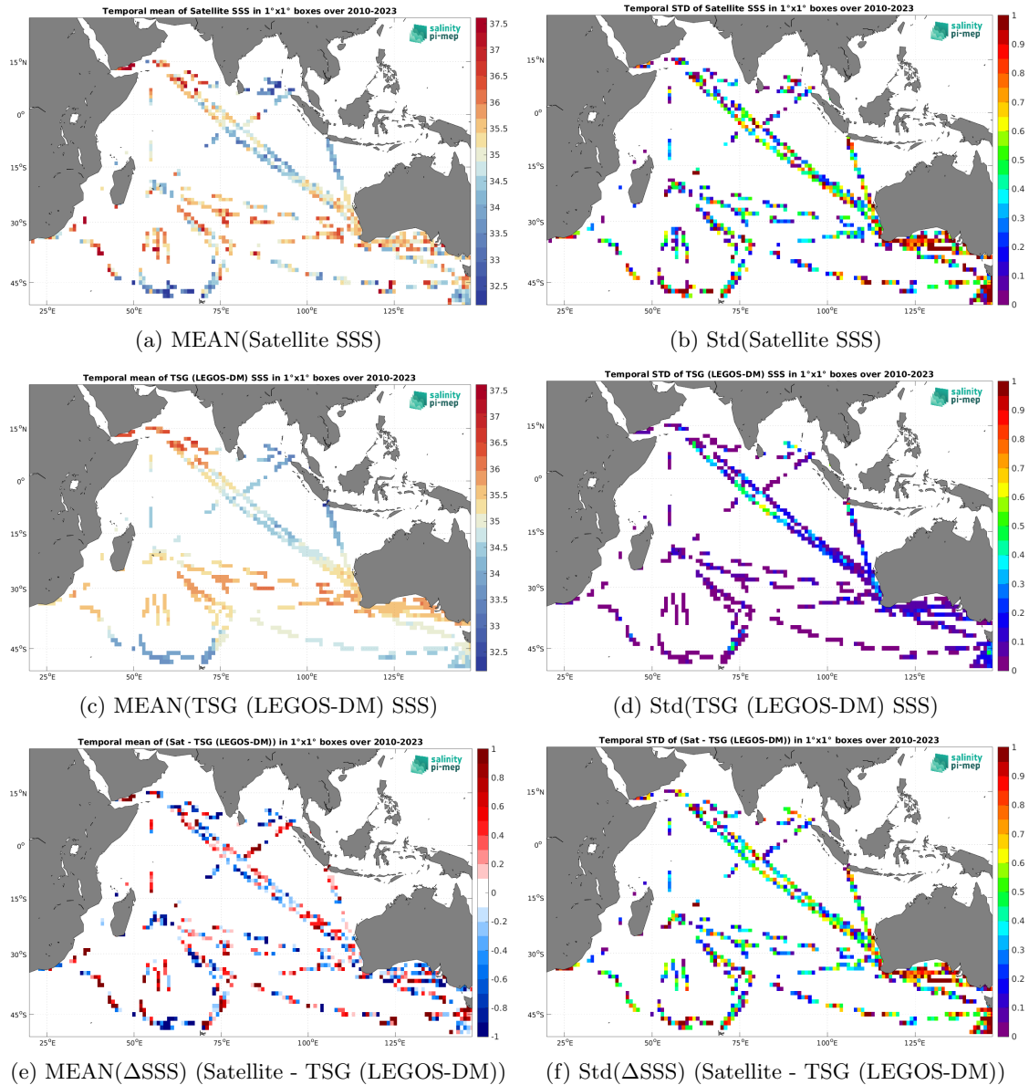
Figure 7: Temporal mean (left) and Std (right) of SSS from SMOS SSS L2 v700 (ESA) (top), TSG (LEGOS-DM) (middle), and of \Delta SSS (Satellite - TSG (LEGOS-DM)). Only match-up pairs are used to generate these maps.
