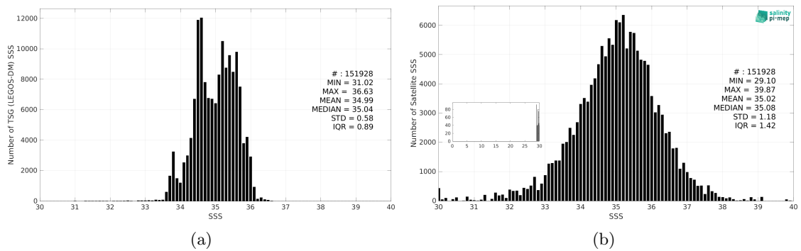
Figure 3: Histograms of SSS from TSG (LEGOS-DM) (a) and SMOS SSS L2 v700 (ESA) (b) considering all match-up pairs per bins of 0.1 over the Indian Ocean Pi-MEP region and for the full satellite product period.
