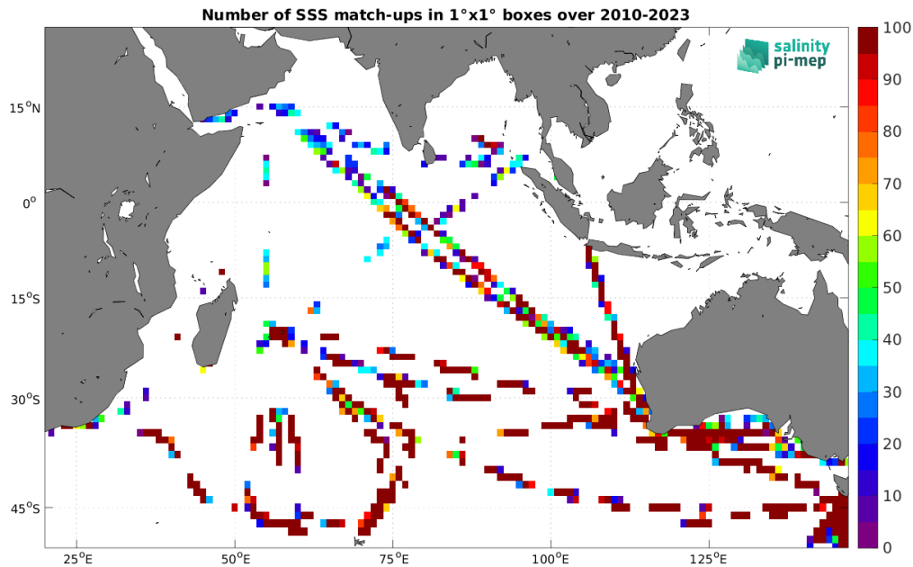
Figure 5: Number of SSS match-ups between TSG (LEGOS-DM) SSS and the SMOS SSS L2 v700 (ESA) SSS product for the Indian Ocean Pi-MEP region over 1^\circ \times 1^\circ boxes and for the full satellite product period.
