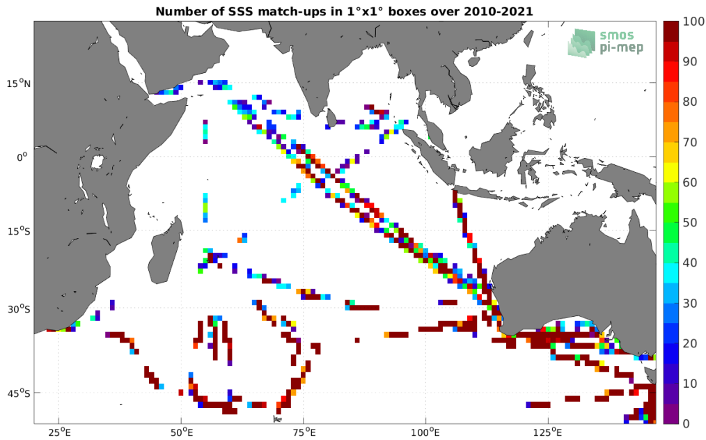
Figure 4: Number of SSS match-ups between TSG (LEGOS-DM) SSS and the SMOS SSS L2 v700 (ESA) SSS product for the Indian Ocean Pi-MEP region over 1^\circ \times 1^\circ boxes and for the full satellite product period.
