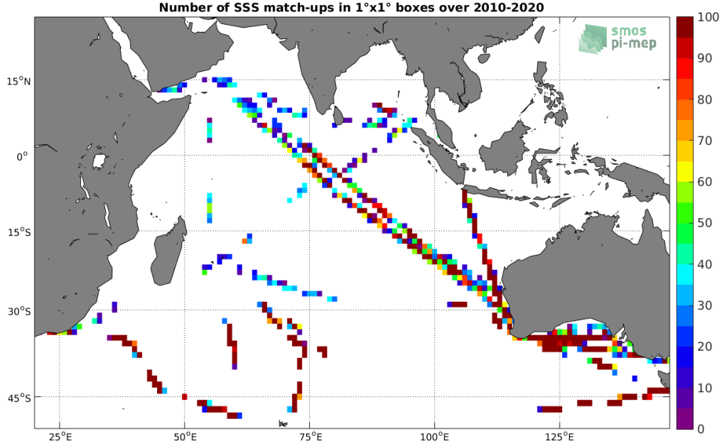
Figure 4: Number of SSS match-ups between TSG (LEGOS-DM) SSS and the SMOS SSS L2 v700 (ESA) SSS product for the Indian Ocean Pi-MEP region over 1^\circ \times 1^\circ boxes and for the full satellite product period.
