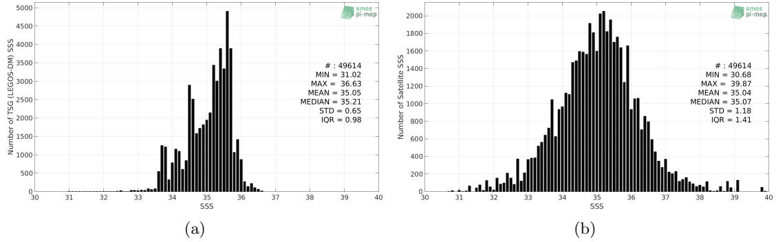
Figure 2: Histograms of SSS from TSG (LEGOS-DM) (a) and SMOS SSS L2 v700 (ESA) (b) considering all match-up pairs per bins of 0.1 over the Indian Ocean Pi-MEP region and for the full satellite product period.
