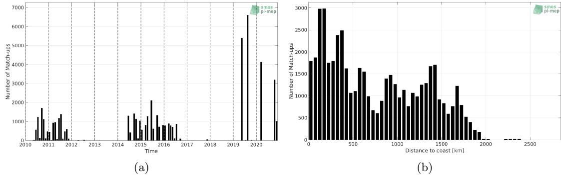
Figure 1: Number of match-ups between TSG (LEGOS-DM) and SMOS SSS L2 v700 (ESA) SSS as a function of time (a) and as function of the distance to coast (b) over the Indian Ocean Pi-MEP region and for the full satellite product period.
