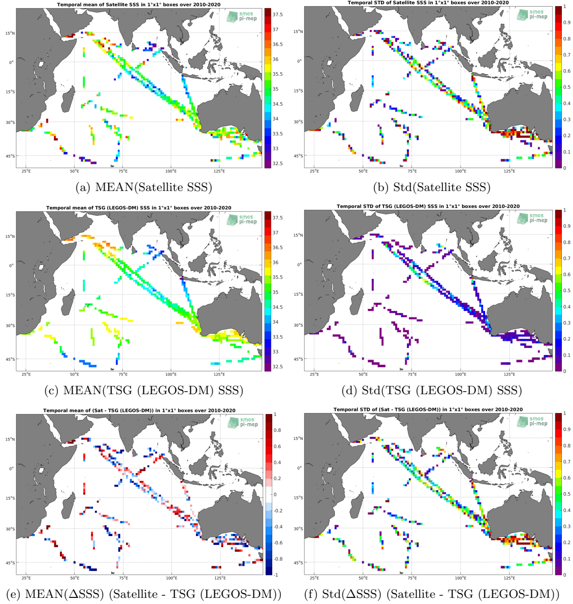
Figure 6: Temporal mean (left) and Std (right) of SSS from SMOS SSS L2 v700 (ESA) (top), TSG (LEGOS-DM) (middle), and of \Delta SSS (Satellite - TSG (LEGOS-DM)). Only match-up pairs are used to generate these maps.
