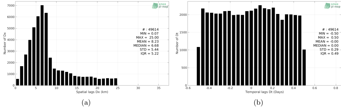
Figure 5: Histograms of the spatial (a) and temporal (b) lags between the location/time of the TSG (LEGOS-DM) measurement and the date of the corresponding SMOS SSS L2 v700 (ESA) SSS pixel.
