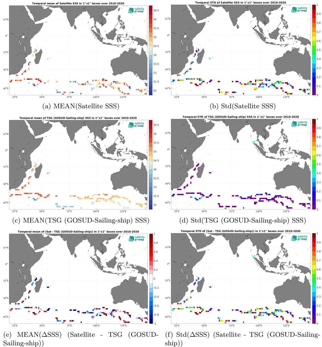
Figure 7: Temporal mean (left) and Std (right) of SSS from SMOS SSS L2 v700 (ESA) (top), TSG (GOSUD-Sailing-ship) (middle), and of \Delta SSS (Satellite - TSG (GOSUD-Sailing-ship)). Only match-up pairs are used to generate these maps.
