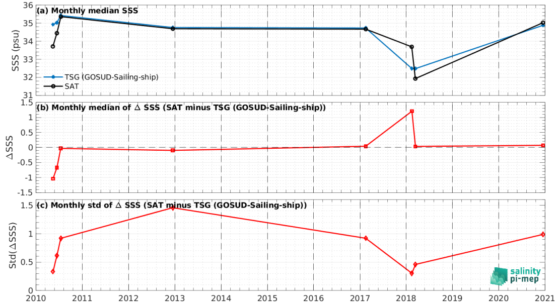
Figure 8: Time series of the monthly median SSS (top), median of \Delta\text{SSS} (Satellite - TSG (GOSUD-Sailing-ship)) and Std of \Delta\text{SSS} (Satellite - TSG (GOSUD-Sailing-ship)) over the Indian Ocean Pi-MEP region considering all match-ups collected by the Pi-MEP.
