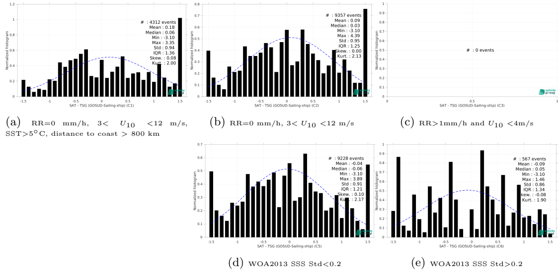
Figure 15: Normalized histogram of \Delta SSS (SMOS SSS L2 v700 (ESA) - TSG (GOSUD-Sailing-ship)) for 5 different subdatasets corresponding to: RR=0 mm/h, 3 < U_{10} < 12 m/s, SST > 5°C, distance to coast > 800 km (a), RR=0 mm/h, 3 < U_{10} < 12 m/s (b), RR > 1mm/h and U_{10} < 4 m/s (c), WOA2013 SSS Std < 0.2 (d), WOA2013 SSS Std > 0.2 (e).
