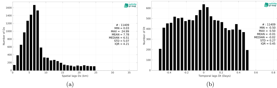
Figure 6: Histograms of the spatial (a) and temporal (b) lags between the location/time of the TSG (GOSUD-Sailing-ship) measurement and the date of the corresponding SMOS SSS L2 v700 (ESA) SSS pixel.
