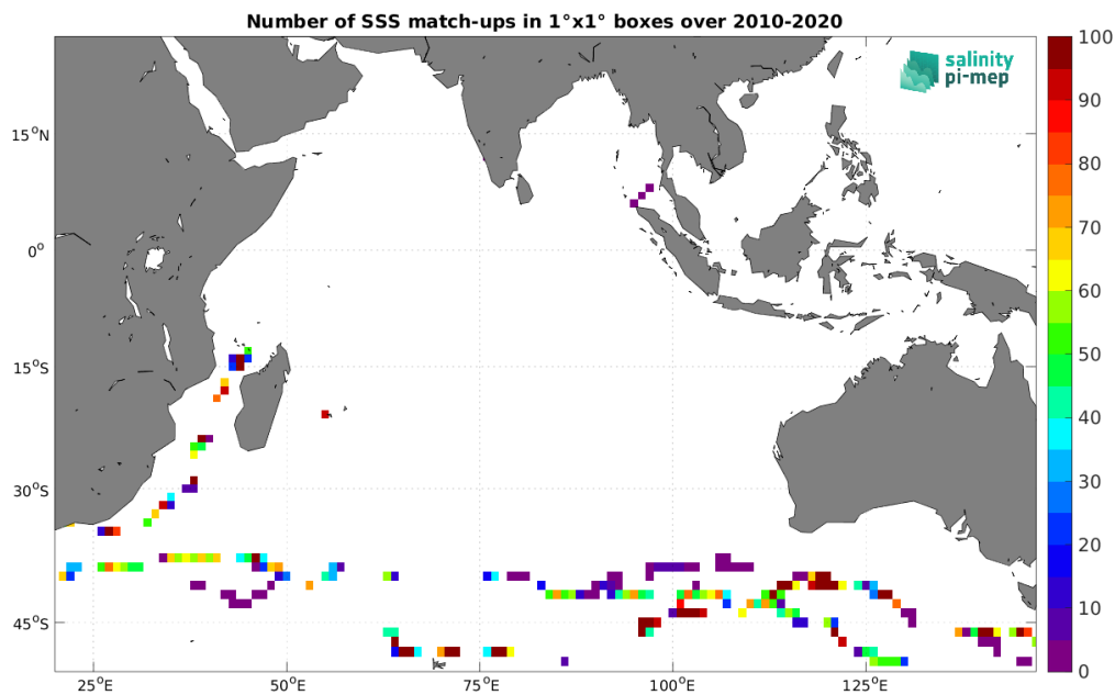
Figure 5: Number of SSS match-ups between TSG (GOSUD-Sailing-ship) SSS and the SMOS SSS L2 v700 (ESA) SSS product for the Indian Ocean Pi-MEP region over 1^\circ \times 1^\circ boxes and for the full satellite product period.
