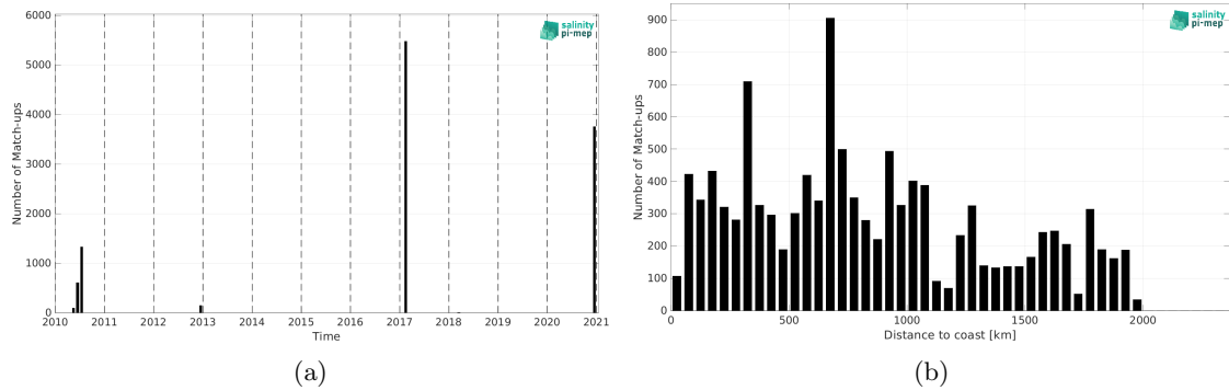
Figure 2: Number of match-ups between TSG (GOSUD-Sailing-ship) and SMOS SSS L2 v700 (ESA) SSS as a function of time (a) and as function of the distance to coast (b) over the Indian Ocean Pi-MEP region and for the full satellite product period.
