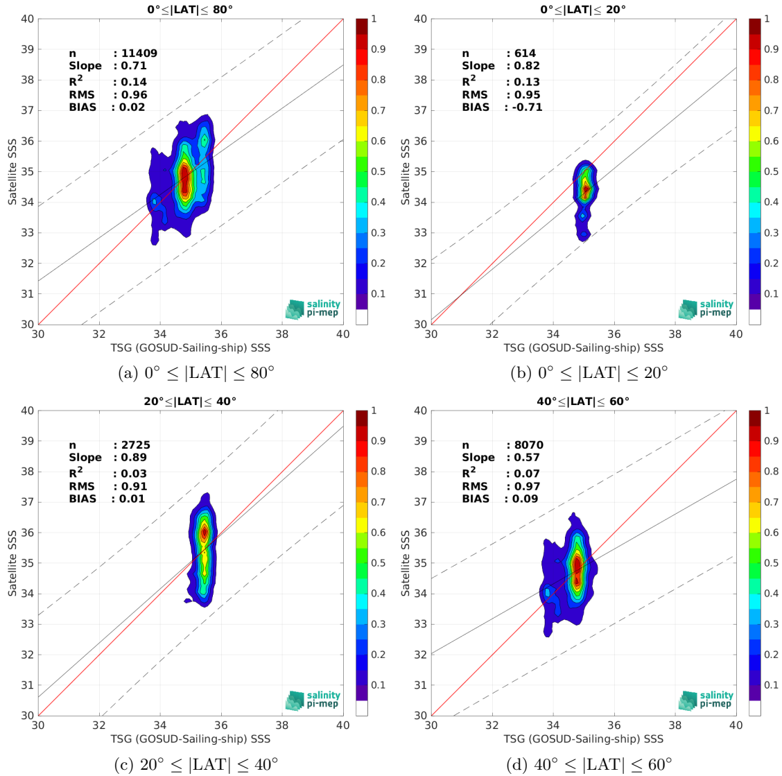
Figure 10: Contour maps of the concentration of SMOS SSS L2 v700 (ESA) SSS (y-axis) versus TSG (GOSUD-Sailing-ship) SSS (x-axis) at match-up pairs for different latitude bands. For each plot, the red line shows x=y . The black thin and dashed lines indicate a linear fit through the data cloud and the \pm 95\% confidence levels, respectively. The number match-up pairs n , the slope and R^2 coefficient of the linear fit, the root mean square (RMS) and the mean bias between satellite and in situ data are indicated for each latitude band in each plots.
