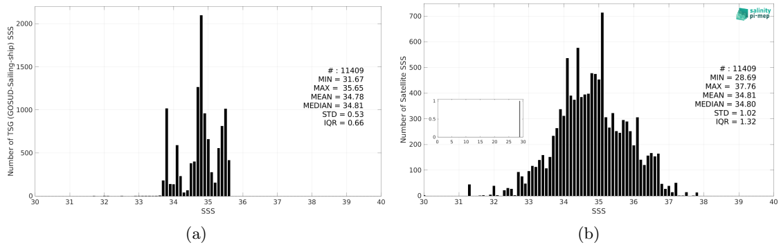
Figure 3: Histograms of SSS from TSG (GOSUD-Sailing-ship) (a) and SMOS SSS L2 v700 (ESA) (b) considering all match-up pairs per bins of 0.1 over the Indian Ocean Pi-MEP region and for the full satellite product period.
