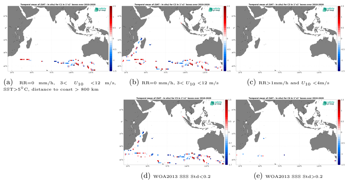
Figure 14: Temporal mean gridded over spatial boxes of size 1^\circ \times 1^\circ of \Delta SSS (SMOS SSS L2 v700 (ESA) - TSG (GOSUD-Sailing-ship)) for 5 different subdatasets corresponding to:RR=0 mm/h, 3 < U_{10} < 12 m/s, SST > 5^\circ\text{C} , distance to coast > 800 km (a), RR=0 mm/h, 3 < U_{10} < 12 m/s (b), RR > 1\text{mm/h} and U_{10} < 4\text{m/s} (c), WOA2013 SSS Std < 0.2 (d), WOA2013 SSS Std > 0.2 (e).
