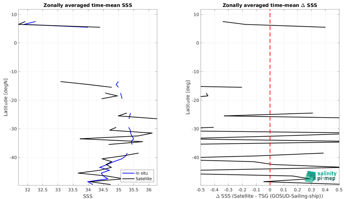
Figure 9: Left panel: Zonal mean SSS from SMOS SSS L2 v700 (ESA) satellite product (black) and from TSG (GOSUD-Sailing-ship) (blue). Right panel: Zonal mean of \Delta SSS (Satellite - TSG (GOSUD-Sailing-ship)) for all the collected Pi-MEP match-up pairs estimated over the full satellite product period.
