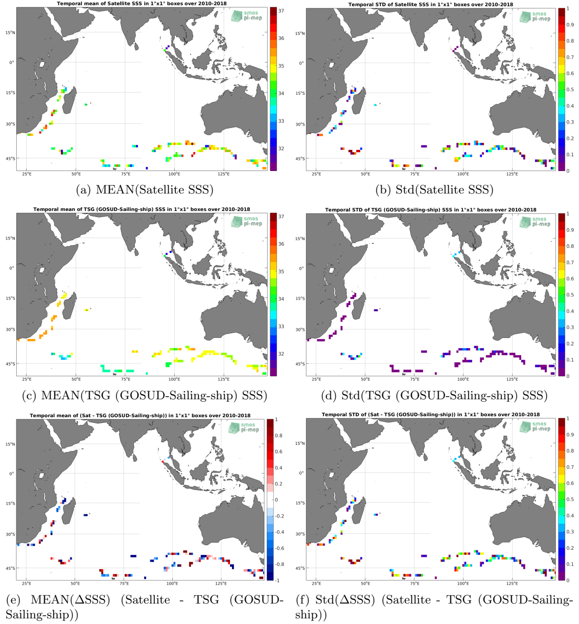
Figure 6: Temporal mean (left) and Std (right) of SSS from SMOS SSS L2 v700 (ESA) (top), TSG (GOSUD-Sailing-ship) (middle), and of \Delta SSS (Satellite - TSG (GOSUD-Sailing-ship)). Only match-up pairs are used to generate these maps.
