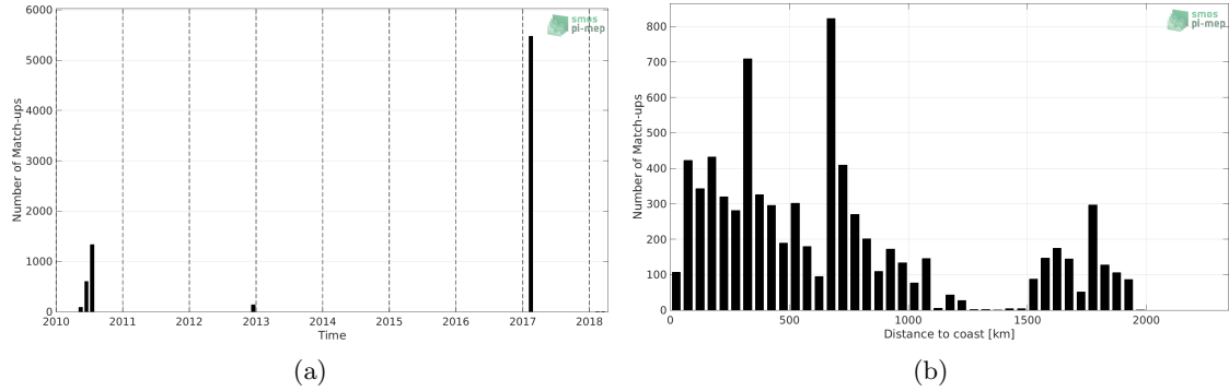
Figure 1: Number of match-ups between TSG (GOSUD-Sailing-ship) and SMOS SSS L2 v700 (ESA) SSS as a function of time (a) and as function of the distance to coast (b) over the Indian Ocean Pi-MEP region and for the full satellite product period.
