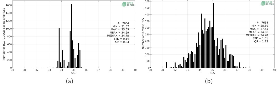
Figure 2: Histograms of SSS from TSG (GOSUD-Sailing-ship) (a) and SMOS SSS L2 v700 (ESA) (b) considering all match-up pairs per bins of 0.1 over the Indian Ocean Pi-MEP region and for the full satellite product period.
