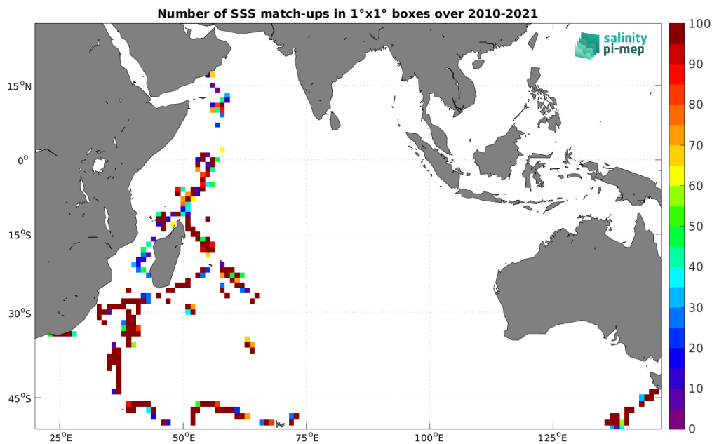
Figure 5: Number of SSS match-ups between TSG (GOSUD-Research-vessel) SSS and the SMOS SSS L2 v700 (ESA) SSS product for the Indian Ocean Pi-MEP region over 1^\circ \times 1^\circ boxes and for the full satellite product period.
