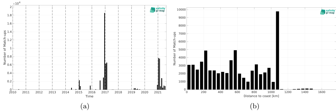
Figure 2: Number of match-ups between TSG (GOSUD-Research-vessel) and SMOS SSS L2 v700 (ESA) SSS as a function of time (a) and as function of the distance to coast (b) over the Indian Ocean Pi-MEP region and for the full satellite product period.
