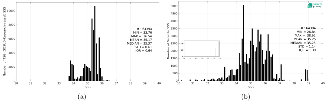
Figure 3: Histograms of SSS from TSG (GOSUD-Research-vessel) (a) and SMOS SSS L2 v700 (ESA) (b) considering all match-up pairs per bins of 0.1 over the Indian Ocean Pi-MEP region and for the full satellite product period.
