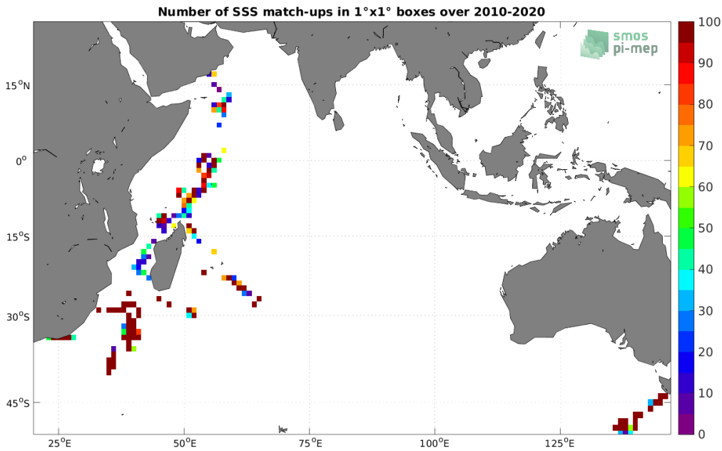
Figure 4: Number of SSS match-ups between TSG (GOSUD-Research-vessel) SSS and the SMOS SSS L2 v700 (ESA) SSS product for the Indian Ocean Pi-MEP region over 1^\circ \times 1^\circ boxes and for the full satellite product period.
